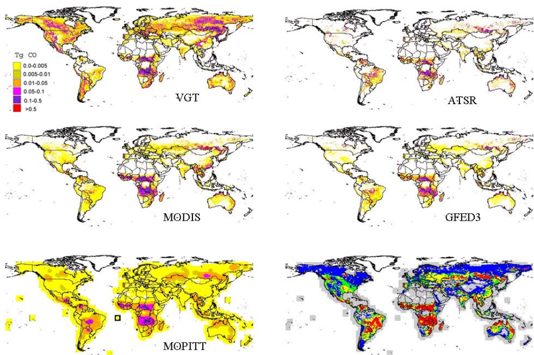
Fig. 1. Maps of CO emissions [Tg] for the year 2003 for 0.5° grid cells; in the right lower corner the map of agreement (i.e. the number of inventories for each cell with CO emissions greater than zero; grey = 1, blue = 2, green = 3, yellow = 4, red = 5). The agreement map has been filtered with a median filter (3 × 3).
