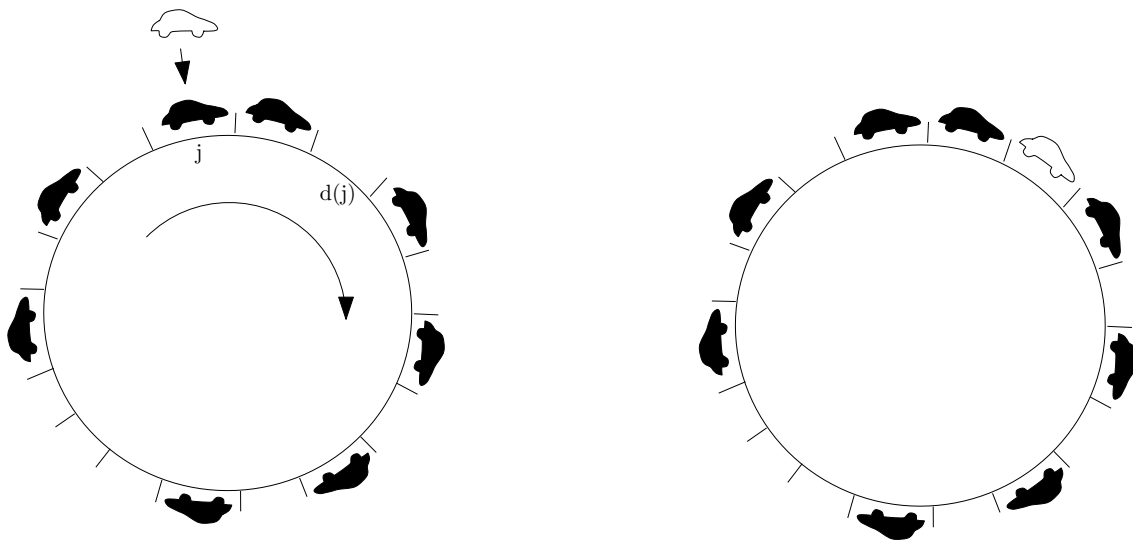
Figure 1 : A car arrives at an occupied site j and parks at the first vacant site d(j) .
