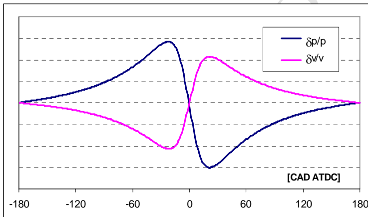
Fig. 5 Qualitative progress of \delta V/V and \delta p/p (obtained using the model described in Appendix A with \delta \vartheta = 1 CAD)
