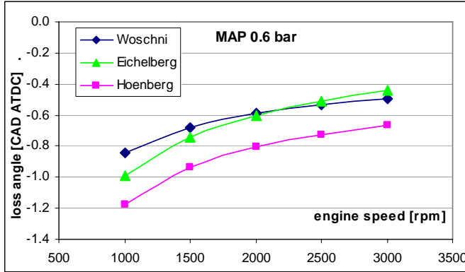
Fig. 10 Comparison between the loss angle values determined at MAP=0.6 bar using the three heat transfer models (engine with \rho=10 )
