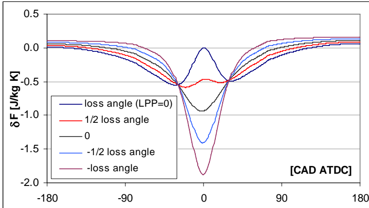
Fig. 6 Loss function variation \delta F for different phase errors (obtained using the model described in Appendix A with \delta\vartheta=1 CAD)
