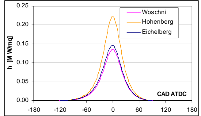
Fig. 11 Heat exchange coefficients according to the three heat transfer models at 2000 rpm and MAP=0.6 bar (engine with \rho=10 )
