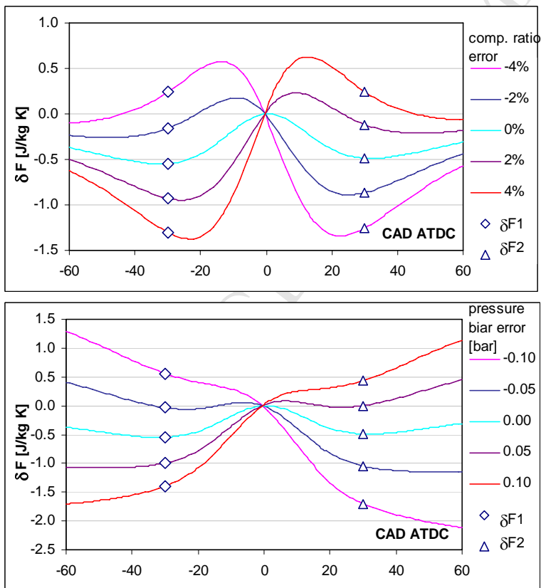
Fig. 7 Loss function variation \delta F in presence of compression ratio error (top) and pressure bias error (bottom): \delta F_1 ( \diamond ) and \delta F_2 ( \Delta ) are shown (pressure cycles phased with LPP=0 obtained using the model described in Appendix A with \delta\vartheta=1 CAD)
