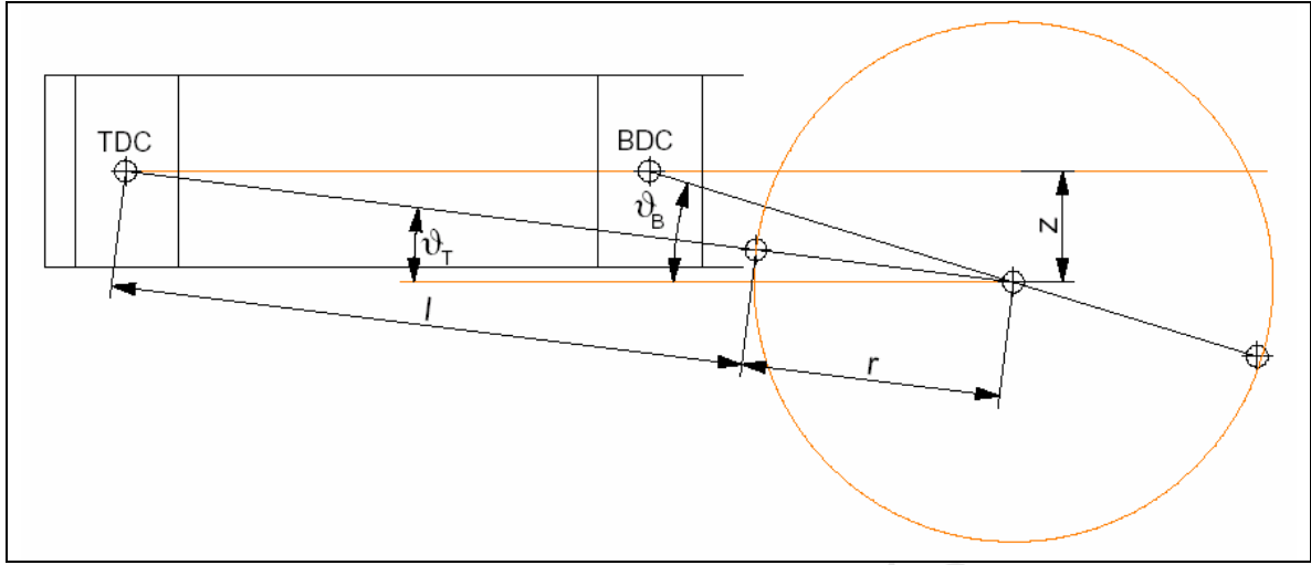
Fig. 14 Representation of a non centred crank mechanism
