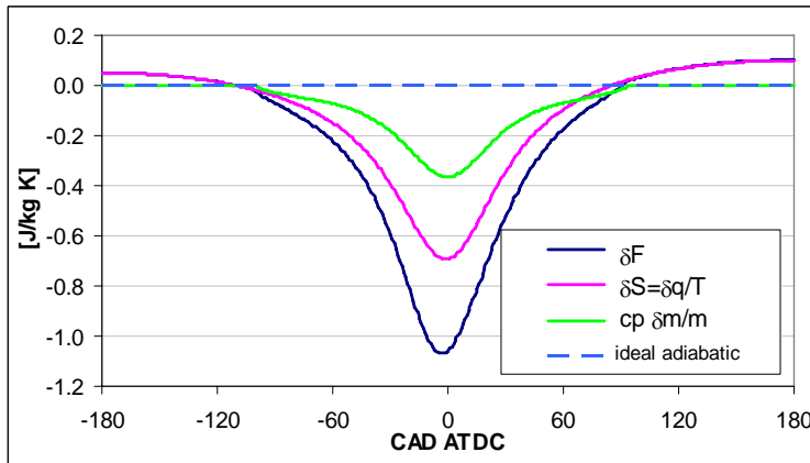
Fig. 4 Loss function variation \delta F and its two constitutive terms (obtained using the model described in Appendix A with \delta \vartheta = 1 CAD)
