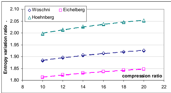
Fig. 15 Entropy variation ratio as function of compression ratio for three different heat transfer models
