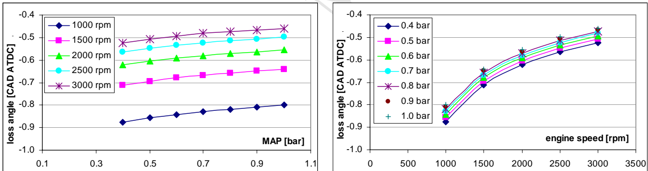
Fig. 9 Loss angle value determined with compression ratio \rho=10 using the Woschni heat transfer model
