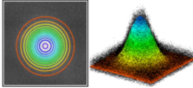
Figure 5 : Image on the CCD camera of the fundamental mode exiting the fiber (black and white) at \lambda = 951\text{nm} , with a 2D gaussian curve fit (color).
