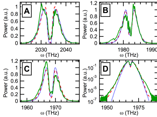
Figure 6 : Measured transmitted spectrum at different wavelengths at maximum pump power (green line): A: 926.8nm ( \tau=0.794\text{ps} ), B: 950.8nm ( \tau=0.934\text{ps} ), C: 957.7nm ( \tau=0.934\text{ps} ), D corresponds to C presented in Log scale. The spectra are compared with the spectra calculated using expression (9) (blue dotted curves) and spectra given by the numerical Split Step Fourier Model taking into account the measured dispersion of the fiber (red dashed line). The pulse durations are deduced from the autocorrelation measurement.
