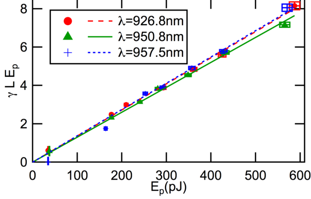
Figure 8 : Plot of the nonlinear coefficient determined by fitting the transmitted spectrum as a function of the energy of the pulse with measurements at three different wavelengths.
