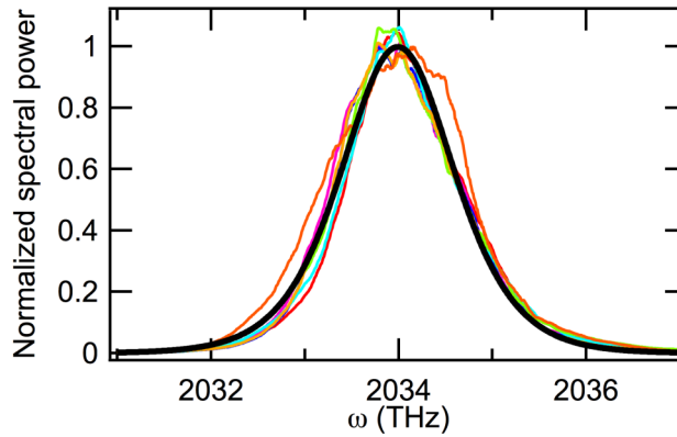
Figure 3 : Comparison between a batch of experimental spectra obtained with identical operating conditions for the laser ( \lambda=926.8\text{nm} ) and the theoretical spectrum calculated using Eq. (11) and the value of \tau=0.794\text{ps} deduced from the autocorrelation measurement.
