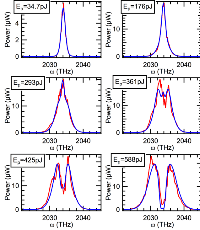
Figure 7 : Spectra of the pulses (red curve) transmitted through the liquid filled hollow core fiber and the fit (blue curve) with Eq. (9) at different incident pulse energies in the fiber at a wavelength of 926.8nm (the incident spectra are the ones shown in Fig. 3).
