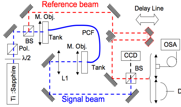
Figure 2 : Schematic experimental set-up. BS: beam splitter cube, \lambda/2 : Half wave plate, Pol.: Polarizer, M.Obj.: x6.3 microscope objective, D: Detector, OSA: Optical spectrum analyzer, PCF: Liquid filled hollow core photonic crystal fiber.
