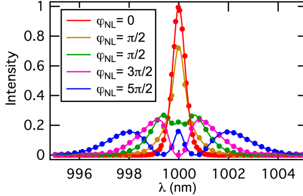
Figure 1 : Calculated intensity spectrum of a secant hyperbolic pulse through a 1m nonlinear fiber, for different values of the nonlinear phase shift (absorption is neglected for simplicity). The solid lines correspond to the analytical model (Eq. (9)) and the markers to the numerical simulation using the split step Fourier method.
