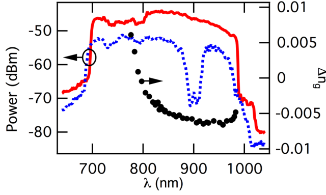
Figure 4 : Power of a supercontinuum source transmitted through the HC-1550-02 hollow core fiber filled with acetone (blue dotted curve) and acetone-d6 (red line). The additional losses due to overtones of IR absorption bands of acetone are eliminated by deuteration, giving a full transmission band for the acetone-d6 filled fiber. The shift of the lower edge of the transmission band of the fiber filled with acetone-d6 is due to the slightly lower index of acetone-d6 compared to non-deuterated acetone [25]. The black dots show the measured variation of the group index of the fiber, from which the dispersion is deduced.
