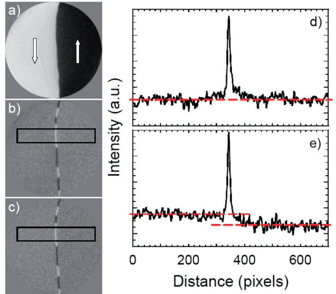
Fig. 4. (Color online) Magnetic domains and domain walls in a 3 nm-thick Fe film grown on a W(110) single crystal. Field of view is 5 \mu\text{m} . (a) The spin polarization of the incident electron beam is aligned along the direction of magnetization (white arrows) in the Fe film ( [1-10] direction). (b, c) The incident spin polarization is rotated by 90^\circ and 89^\circ respectively to spatially resolve the internal chirality of the 180^\circ domain wall. (d, e) Intensity profiles across the 180^\circ domain wall, averaged within the black frames shown in (b, c). Although no obvious contrast is observed in (b, c) between the two magnetic domains, intensity profile reported in (e) clearly reveals their orientation, demonstrating in that example that sensitivity to the local direction of magnetization is better than 1^\circ .
