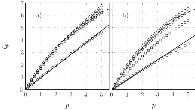
Fig. 3: Structure function exponents, \zeta_p , as a function of p for the synthetic signal (a) and experimental data (b). (o) \zeta_p^{(1)} computed from the first-degree increments; ( \square ) \zeta_p^{(2)} computed from the second-degree differences and fitted by (—) \zeta_p^{(2)} = c_1 p - c_2 p^2/2 with c_1 = 1.92 and c_2 = 0.27 ; ( \diamond ) \zeta_p^{(3)} and ( \triangle ) \zeta_p^{(4)} computed from the third-degree and fourth-degree differences. Solid lines are linear fits of \zeta_p^{(1)} : (a) \zeta_p^{(1)} = 0.95p , and (b) \zeta_p^{(1)} = 0.8p .
