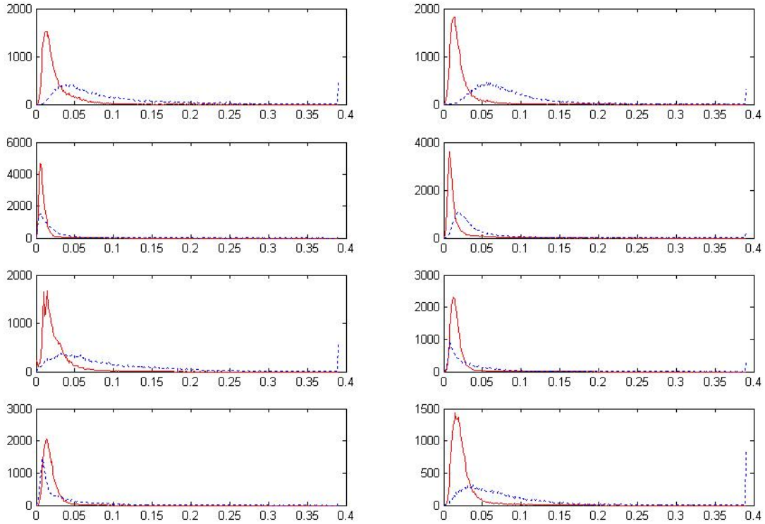
Fig. 4: Gradient magnitude histogram of the eight previous images (Fig. 2) before pre-processing (solid line) and after pre-processing (dotted line).
