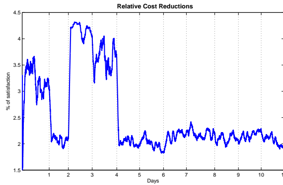
Figure 3: Case N = 4 , \sum_{i=1}^N \beta_i < 1 , 0.2 < \alpha_i \leq 0.8 and r_i^0 = 1/N , 1 \leq i \leq N .
