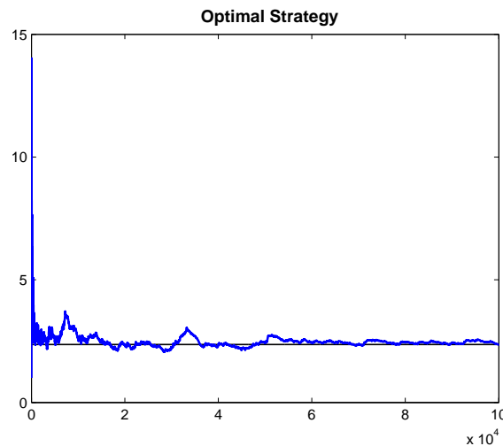
Figure 2: Convergence towards the optimal capacity level of the investment project: \kappa = 1 , \vartheta = 1 , \sigma = 1.5 , \alpha = 0.8 , \beta = 0.7 , c = 0.5 , n = 10^5 , \tilde{\gamma}_n = \frac{5}{n} .
