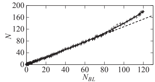
FIG. 5. Experimental determination of the correction to the Beer-Lambert law. The solid curve is a fit to the experimental data with a third-order polynomial, the straight dashed line being the linear contribution. N_{BL} is obtained by using the Beer-Lambert law and summing over transverse pixels in images taken with a nearly resonant probe and a small time of flight of 0.5 ms [see Fig. 4 (a)]. N is obtained from images taken with a probe detuned by 5 MHz and a time of flight of 1.5 ms, for which the Beer-Lambert law is adequate [see Fig. 4 (b)].
