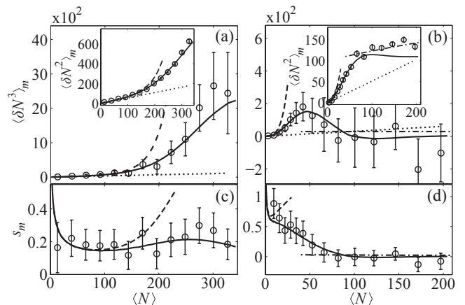
FIG. 2. Measured third moment (open circles) of the atom number fluctuations versus the mean atom number per pixel, for temperatures of 376 nK (a) and 96 nK (b). The insets show the corresponding atom number variances. The error bars are the statistical errors. Graphs (c) and (d) show the skewness s_m corresponding to (a) and (b), respectively. The theoretical predictions, scaled by \kappa_2 = 0.55 and \kappa_3 = 0.34 for (a) and (c), and by \kappa_2 = 0.52 and \kappa_3 = 0.31 for (b) and (d), are shown for comparison: solid lines – the modified Yang-Yang prediction; dashed lines – the ideal Bose gas prediction; dash-dotted lines on (b) and (d) – the quasi-condensate prediction; dotted lines – the shot noise limit \langle N \rangle .
