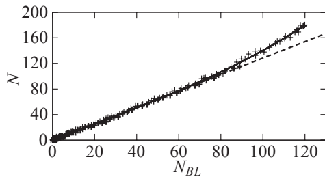
FIG. 6: Experimental determination of the correction to the Beer-Lambert law. The solid curve is a fit to the experimental data with a third-order polynomial, the straight dashed line being the linear contribution. N_{BL} is obtained by using the Beer-Lambert law and summing over transverse pixels in images taken with a nearly resonant probe and a small time of flight of 0.5 ms [see Fig. 5 (a)]. N is obtained from images taken with a probe detuned by 5 MHz and a time of flight of 1.5 ms, for which the Beer-Lambert law is adequate [see Fig. 5 (b)].
