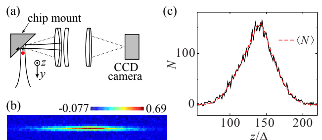
FIG. 1: (Color online) (a) Scheme of the absorption imaging setup. The probe laser beam crosses the atomic cloud (shown as a red dot) before its reflection from the chip surface and detection on a CCD camera. (b) A typical in-situ absorption image, with the scale on the colorbar corresponding to the optical density. The pixel size in the object plane is \Delta = 4.5 \mu\text{m} . (c) A typical longitudinal density profile (solid curve), together with the mean profile (dashed red curve).
