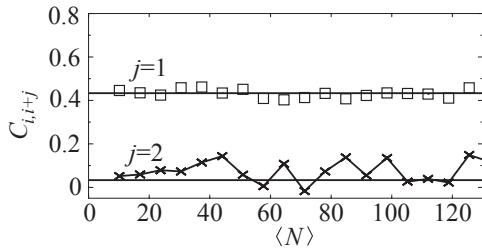
FIG. 3: Correlation of atom number fluctuations between adjacent (open squares) and next-neighbor (crosses) pixels. The solid lines are the predictions for an impulse response function with an rms width of 2.0 \mu\text{m} , obtained by fitting C_{i,i+1} .
