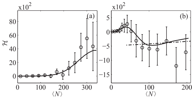
FIG. 4: The measured three-body integral \mathcal{H}_m versus \langle N \rangle , corresponding to the data of Figs. 2 (a) and (b), respectively. The solid (dash-dotted) curves are the thermodynamic predictions from the modified Yang-Yang (quasi-condensate) model.
