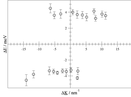
Figure 2. Dispersion relation of the observed surface BP. Data points were obtained from fittings of \rho_{zz}/\rho_{Debye} with two Gaussian functions, see Fig. 1.
