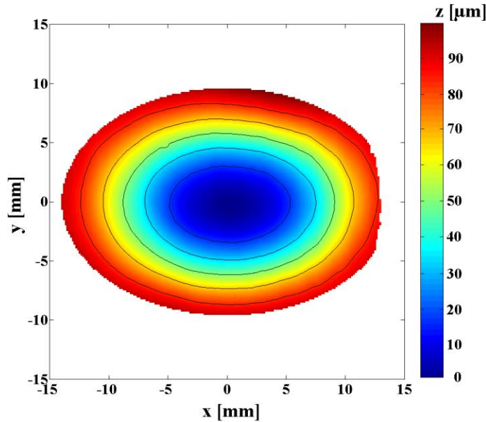
Figure 4. Mirror profile measured in the profilometer [32] for a uniform applied voltage of 2700 V at the 5 electrodes. The x axis is along the major axis of the sapphire clamping aperture (see figure 3), the y axis along the minor axis and the wafer deflection is displayed in the z axis. (x, y, z) are the mirror coordinates of figure 2 (b).
