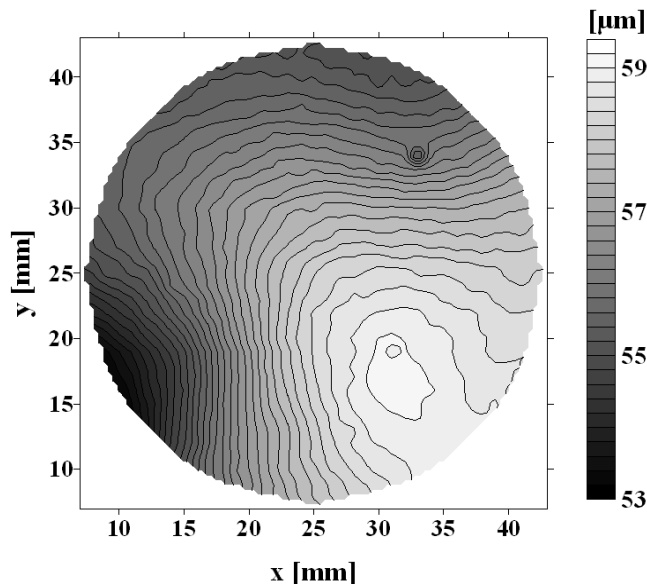
Figure 6. Thickness map of the used Si(111) wafer used in this experiment. The thickness map was recorded using the instrument described in [37].
