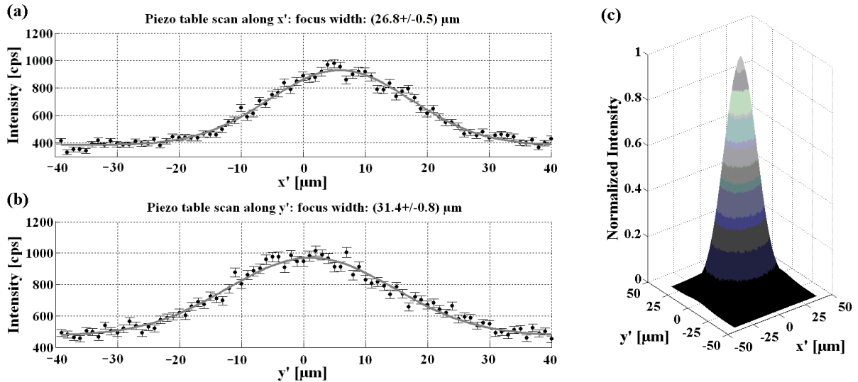
Figure 5. In (a) and (b) the measured He intensities are presented (circles) with a fit (grey line) to determine the actual best full width at half maximum. These scans were done with slits in the piezo table along the axes x' and y' . In (c) the best helium beam focus is shown in a three-dimensional representation. The voltage applied to all electrodes was 2760 V.
