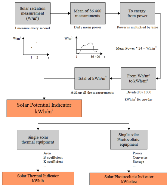
Figure 12. Solar potential estimation.
