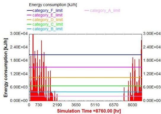
Figure 2. Energy consumption compared to energy performance categories.
