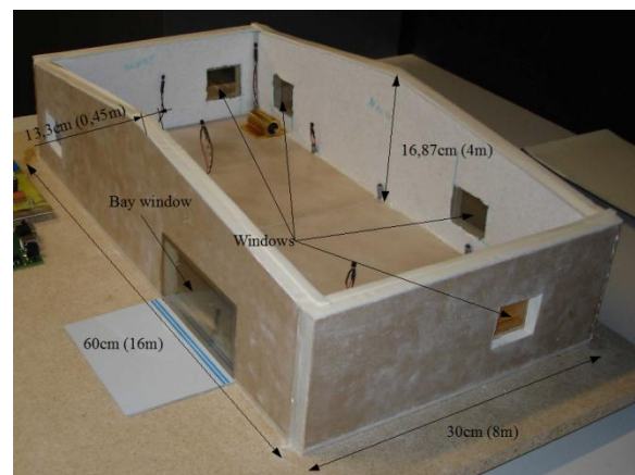
Figure 7. The building mock-up.
