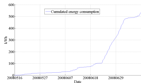
Figure 11. Cumulated energy consumption of the air conditioning system.
