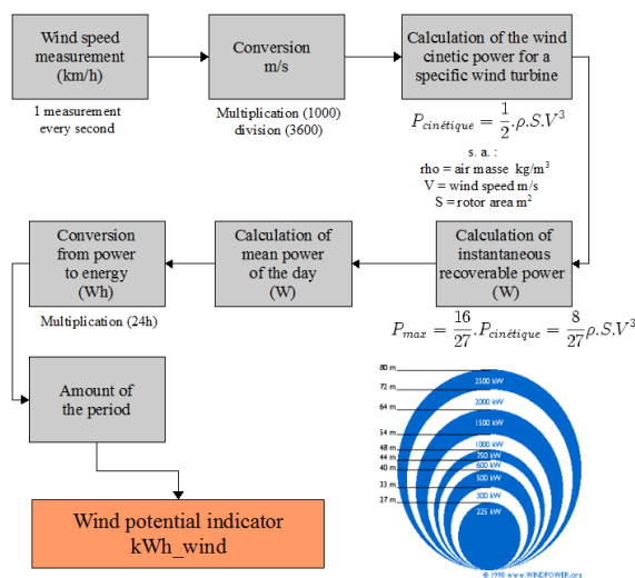
Figure 13. Wind potential estimation.
