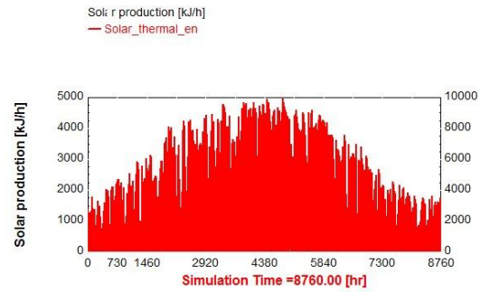
Figure 3. Solar thermal energy production.
