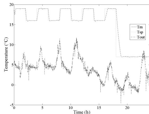
Figure 14. Heating control with MPC scheme.
