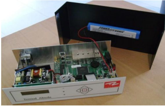
Figure 4. BEMS prototype.
