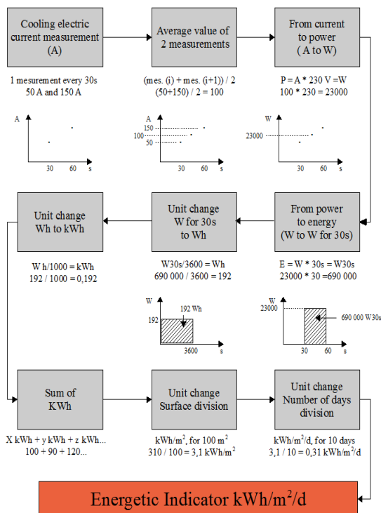
Figure 9. Air-conditioning consumption algorithm.
