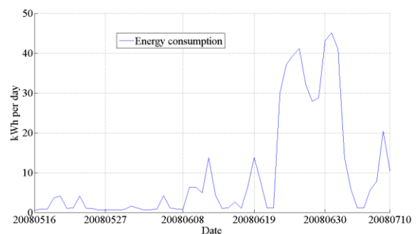
Figure 10. Daily energy consumption of the air-conditioning system.
