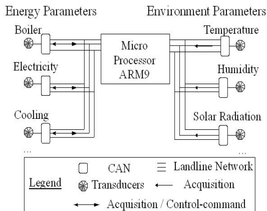
Figure 5. BEMS communication scheme.
