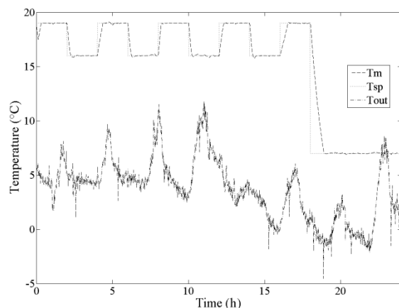
Figure 14. Heating control with MPC scheme.
