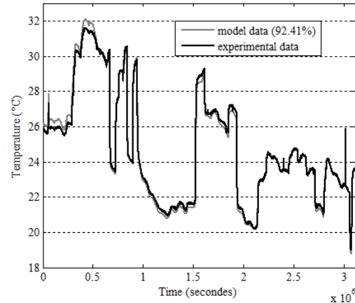
Figure 2. Comparison of experimental and model data for South West temperatures.
