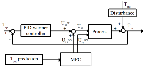
Figure 5. MPC control framework.
