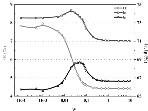
Figure 12. Influence of the constraint applied to W_{FE} .
