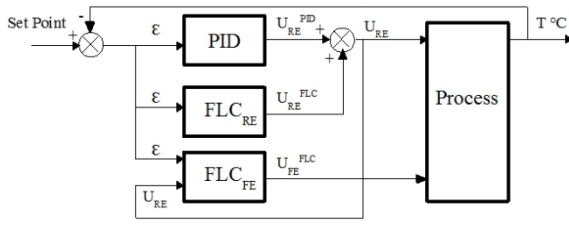
Figure 6. FLC control framework.
