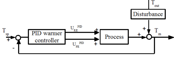
Figure 4. PID control framework.
