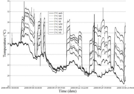
Figure 1. Mock-up temperatures acquisition.
