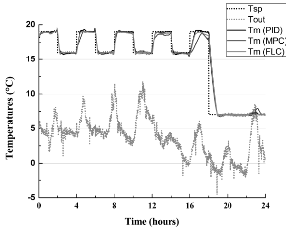
Figure 11. Simulation of indoor temperature.
