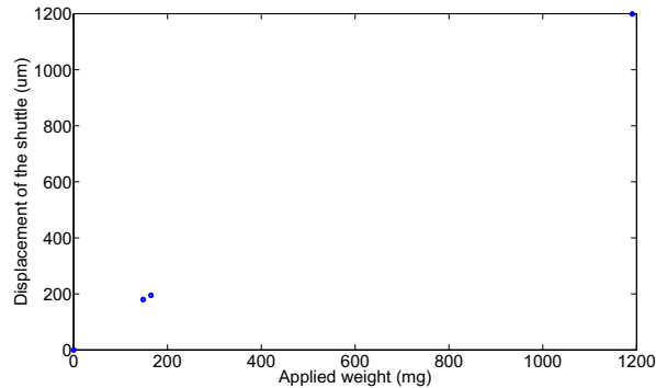
Figure 7. The displacement versus applied load used to calibrate the auxiliary cantilever.
