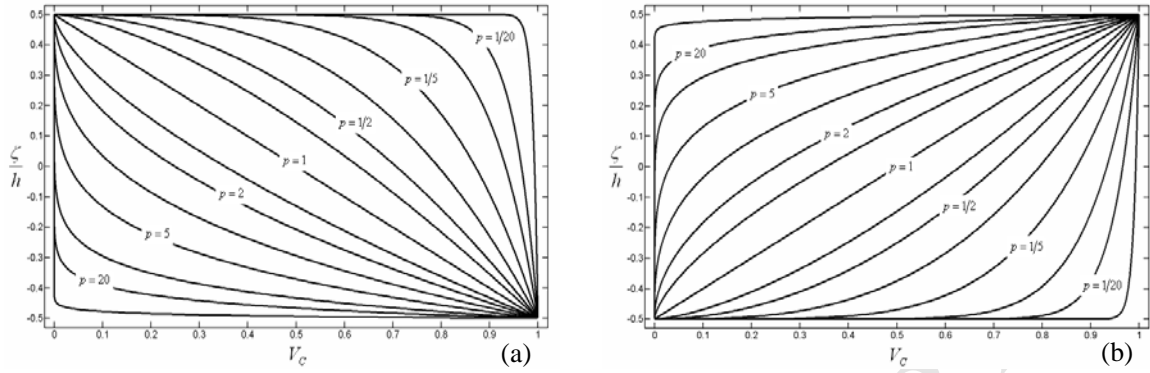
Figure 3. Variations of the ceramic volume fraction V_c through the thickness for different values of the power-law index p : (a) FGM_{1(a=1/b=0/c/p)} , (b) FGM_{2(a=1/b=0/c/p)} .
