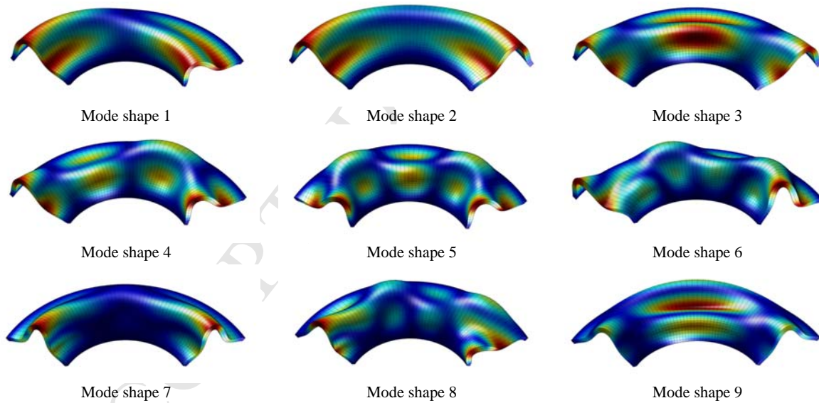
Figure 7. Mode shapes for the FGM_1 ( a=1/b=0.5/c=2/p=1 ) toro-parabolic panel C-F-C-F.
