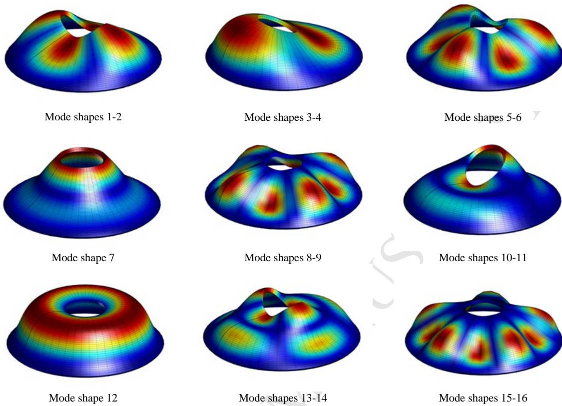
Figure 10. Mode shapes for the FGM_{1(a=0.8/b=0.2/c=3/p=1)} parabolic dome C-F.
