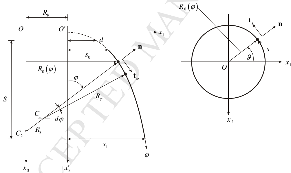
Figure 2. Shell geometry.
