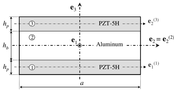
Fig. 2. Three-layered sandwich piezoelectric beam: cross-section.
