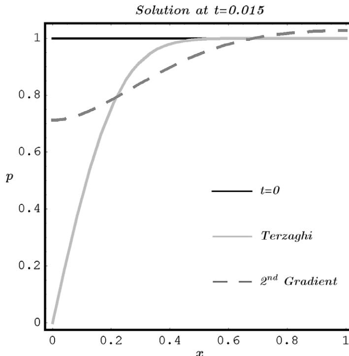
Fig. 2. Late time fluid pressure profile obtained by classical consolidation theory (solid line) and second gradient theory (dashed line). The initial value of the fluid pressure is also depicted (black line). A fluid overpressure at the impermeable wall arises. Dimensionless time value is explicitly indicated.
