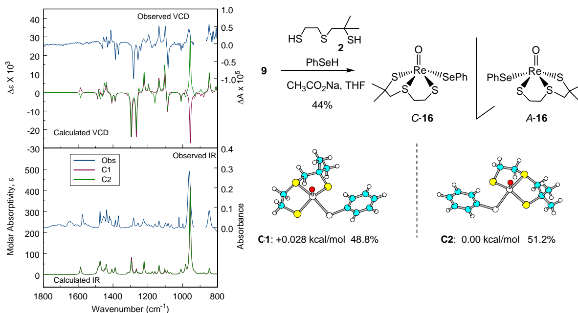
Figure 8: Optimized geometries, relative energies and Boltzmann populations (23°C) for conformers C1 and C2 of complex \text{ECD}_{220}(+)\text{-16} . Comparison of infrared (lower frame) and VCD (upper frame) spectra observed for complex \text{ECD}_{350}(+)\text{-16} in \text{CDCl}_3 solvent (right axes) with calculated spectra (left axes) for the two stable conformations, C1 and C2, with geometries and C- \text{ECD}_{220}(+)\text{-16} absolute configuration.
