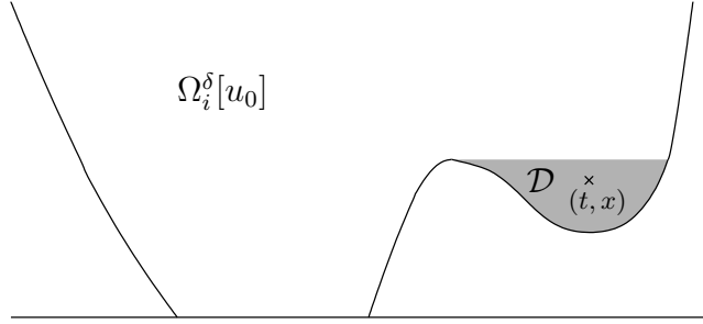
Figure 1: An example of the set \Omega_i^\delta[u_0] . The point (x, t) \in \Omega_i^\delta[u_0] can not be connected to 0 by a trajectory (x(s), s) staying within \Omega_i^\delta[u_0] . More generally, for the points in the hatched area, called \mathcal{D} , there is no admissible trajectory. We have indeed \mathcal{C}_{i+1}^\delta[u_0] = \Omega_i^\delta[u_0] \setminus \mathcal{D} .
