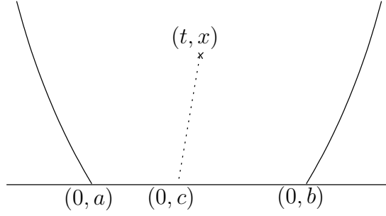
Figure 2: The case with R(x) = R a positive constant, \{x \in \mathbb{R} \mid u_0(x) > u_m\} = (a, b) and u_0(\cdot) \geq u_m on an interval [a, b] . The set \Omega is a union of hyperbolas. The optimal trajectories are straight lines and we have U(x, t) = -\frac{|x-c|^2}{4t} + Rt + u_0(c) , where c is a point where the maximum in (48) is attained.
