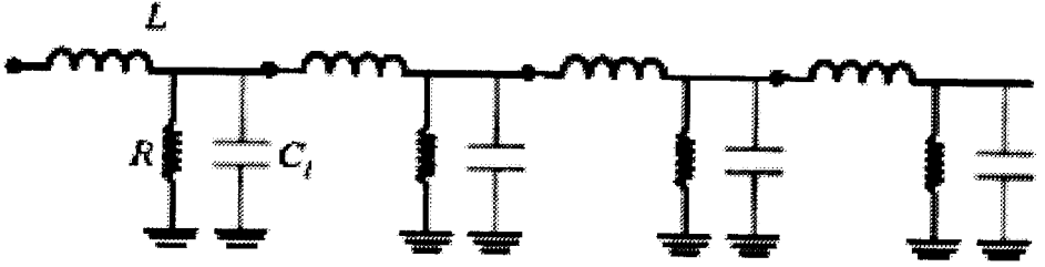
Fig. 2. Standard second order transmission line
