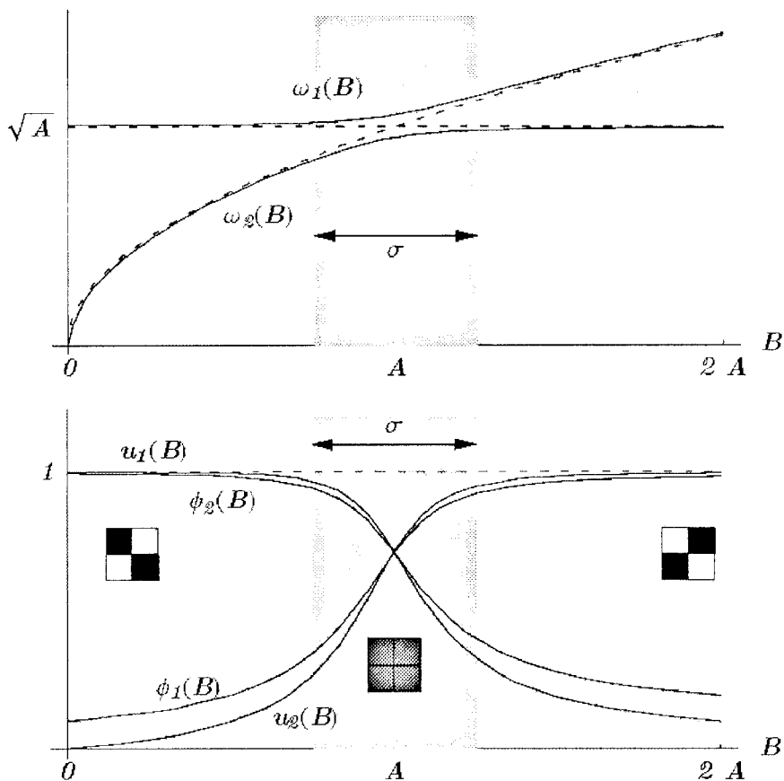
Fig. 7. Behavior of eigenfrequencies and eigenvectors near veering
