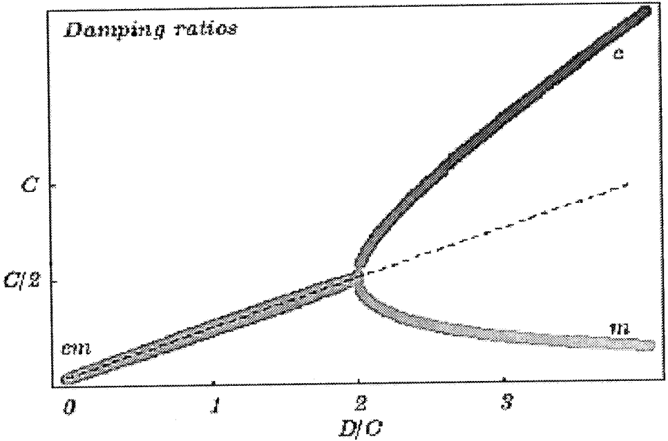
Fig. 9. Damping ratios versus D/C for B = A
