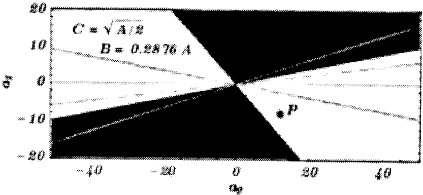
Fig. 14. Regions of instability (black) and stationary solutions (for B < A )
