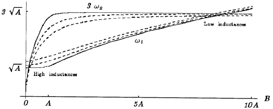
Fig. 13. Solutions for the three-to-one resonance in terms of inductance
