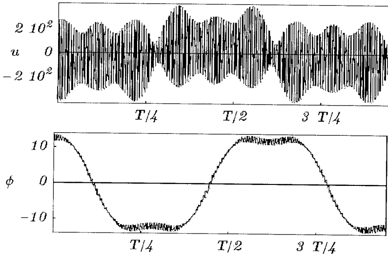
Fig. 17. Time evolution of u and \phi with initial conditions in P ( C = \sqrt{A/2} , B = 0.288A )
