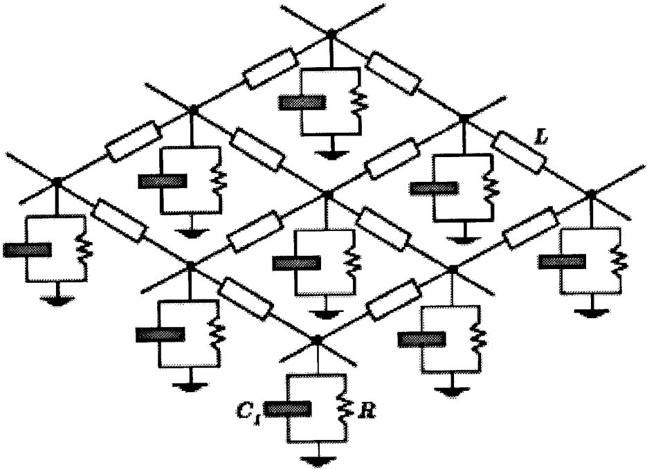
Fig. 4. Second order transmission net
