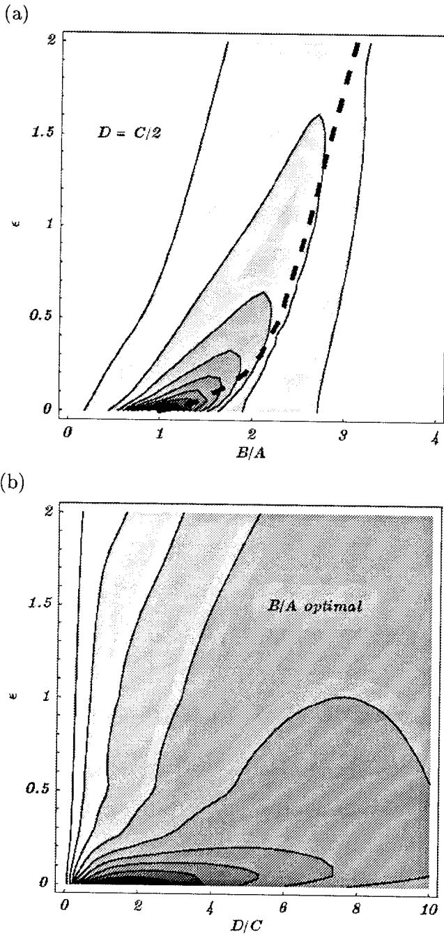
Fig. 11. Energy dissipation as function of (a) B/A and \epsilon ; (b) D/C and \epsilon . In the darker regions the dissipation is higher
