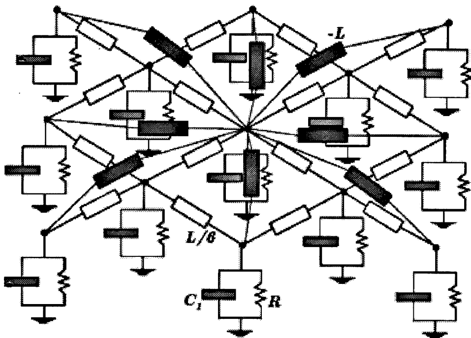
Fig. 5. Fourth order transmission net
