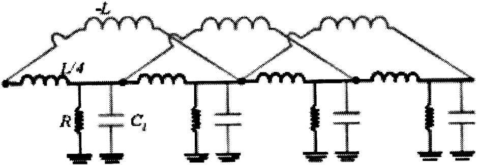
Fig. 3. Fourth order transmission line
