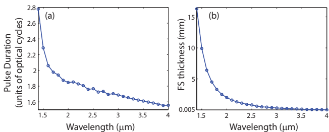
Figure 8. (Color online). (a) Temporal duration (in cycle unit) at different wavelengths of pulses compressed with an optimal FS thickness. Best FS thicknesses are displayed in (b). Not that the CaF 2 exit window is taken into account.
