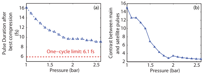
Figure 6. (Color online). Pressure dependence of (a) minimal pulse duration achievable by compression with optimized FS thickness in each case and (b) ratio between main and satellite pulse intensities.
