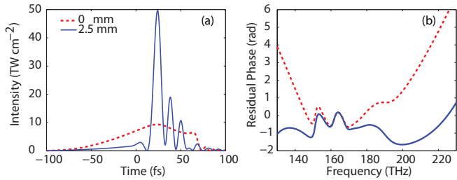
Figure 7. (Color online). (a) Temporal profile and (b) residual spectral phase of the pulse for a pressure of 2.6 bar without (dashed red) and with (blue line) the best compression leading to a FWHM duration of 1.25 cycles.
