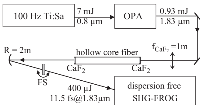
Figure 1. Experimental setup. Idler pulses from a high energy OPA are propagated in a hollow-core fiber filled with 1.4 bar Argon. The broadband pulses are subsequently compressed by linear propagation through a fused silica (FS) plate of 3 mm thickness.
