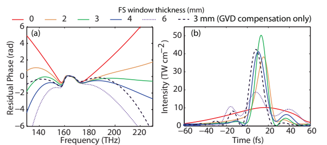
Figure 3. (Color online). Pulse compression for the spectrum of Fig. 2 by adding different amount of FS. The color coding for the spectral phases in (a) corresponds to the temporal intensities in (b). Comparing the green with the black dashed plot demonstrates the effect of uncompensated TOD components.
