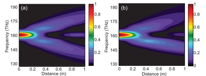
Figure 4. (Color online). Spectral evolution as a function of propagation distance for the simple case considering only n_2 in (a) and for the full model in (b). The latter clearly resembles an asymmetry because of self-steepening, which tends to promote the higher frequency region.
