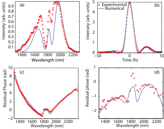
Figure 2. (Color online). Comparison between experimental (red circles) and theoretical (straight blue line) results. (a) Power spectrum for propagation in Argon at pressure of 1.4 bar, (c) spectral phase of the pulse before and (d) after compensation with 3 mm FS. The temporal intensity profile of the compressed pulse is shown in (b).
