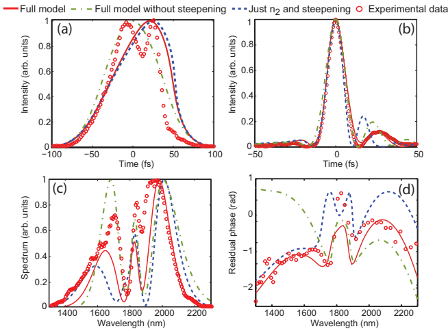
Figure 5. (Color online). Comparison of the three numerical models with experimental measurements. (a) and (b): time profile of (a) the uncompressed and (b) the compressed pulse; (c): broadened power spectrum and (d) its associated phase when the pulse is compressed.
