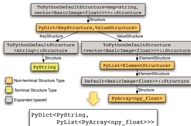
Figure 6 The default Python type when converting from C++ to Python is deduced by recursive instantiation of ToPythonDefaultStructure<CPPTyp>.
