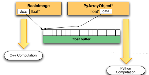
Figure 7 allocate_numpy_array constructs a new Python and C++ array at the same time, to wit, a NumPy array and a BasicImage object. The NumPy array owns the buffer allocated so when its reference count goes to zero, its memory buffer will be freed.
