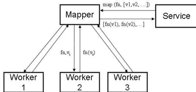
Figure 4: Mapper workflow architecture. fn is the function to be mapped and v_i are the inputs. The function should be stateless, with output depending only on the current input v_i, not on the previous inputs.
