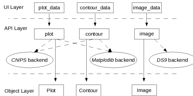
Figure 5. Sherpa Visualization Interface
