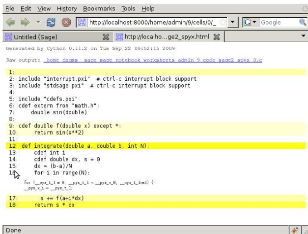
Figure 2 Using the -a switch to the cython command line program (or following a link from the Sage notebook) results in an HTML report of Cython code interleaved with the generated C code. Lines are colored according to the level of “typedness” - white lines translates to pure C without any Python API calls. This report is invaluable when optimizing a function for speed.
