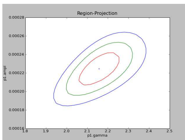
Figure 7. 2D confidence contours, shown here using matplotlib, are a typical product of a Sherpa session. Contours provide the parameter value expectation to some degree of confidence. The smaller the contour, the more constrained the best-fit values are.
