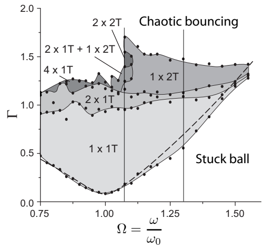
FIG. 4: Experimental phase diagram. The dashed line corresponds to the analytical model for the threshold between a stuck and a bouncing ball. Full lines are guides to the eye. The two gray vertical lines correspond to the bifurcation diagram frequencies in Fig. 3
