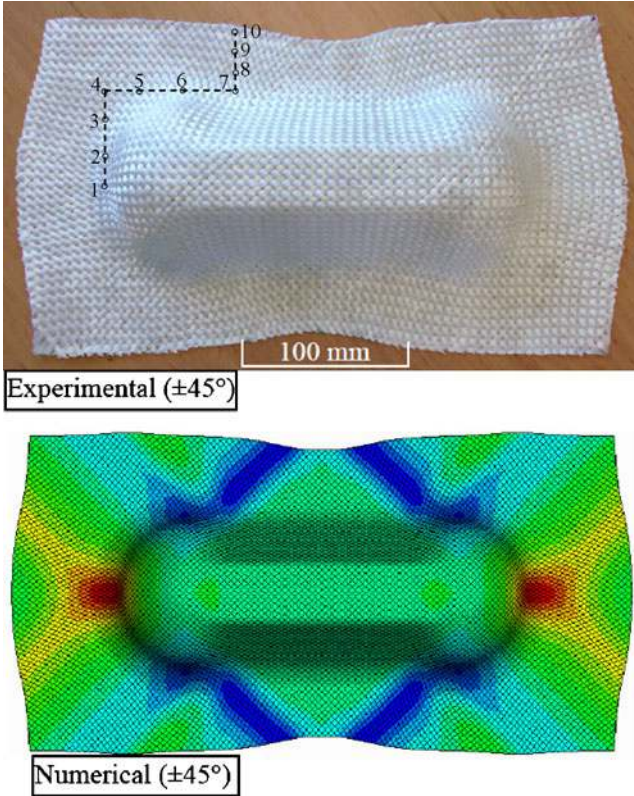
Fig. 5 Experimental and numerical outputs of double dome forming test
