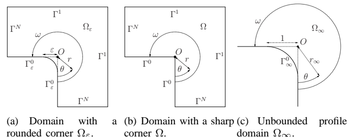
Fig. 1. Considered domains \Omega , \Omega_\infty and \Omega_\varepsilon .
