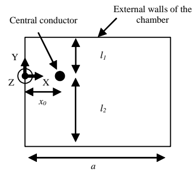
Figure 1. Geometry of a TL in the transverse plane
