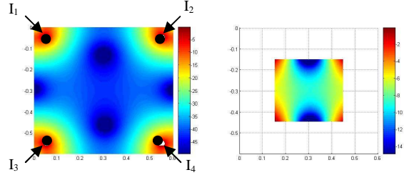
Figure 4. Distribution of the normalized E-field inside the chamber with 4TL excited by I_1=I_2=1 and I_3=I_4=-1
