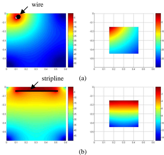
Figure 3. Distribution of the normalized E-field in the transverse plane inside the chamber (on the left) and inside the WA (on the right) in dB: (a) TL with a thin wire conductor (b) stripline used in canonical TEM chambers
