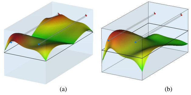
Figure 7. . Distribution of the E-field modulus inside the chamber for differents loads (a) -j500 \Omega load (b) +j500 \Omega load
