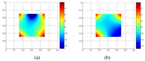
Figure 5. Distribution of the normalized E-field inside the working area for different excitations: (a) I_1=I_2=1, I_3=I_4=-1 (b) I_1=1, I_2=j, I_3=-j, I_4=-1/4
