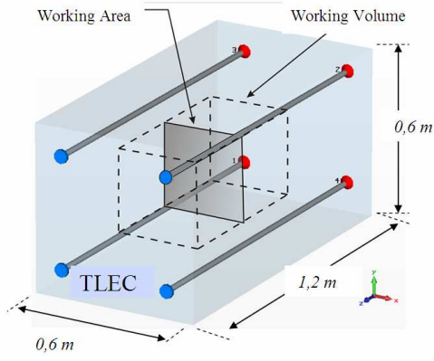
Figure 2. WV and WA definitions in the TLEC
