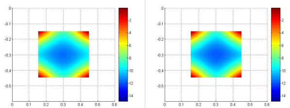
Figure 6. Distribution of the mean normalized E-field inside the working area with an amplitude shifting (on the left) or a phase shifting (on the right)
