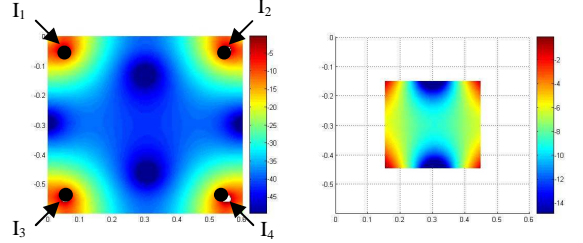
Figure 4. Distribution of the normalized E-field inside the chamber with 4TL excited by I_1=I_2=1 and I_3=I_4=-1
