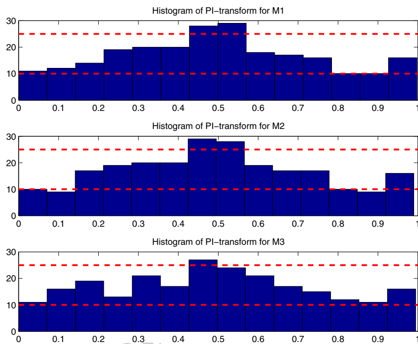
Fig. 2. Histograms of probability integral transforms z_t
