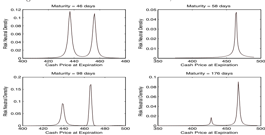
Fig. 5. Estimated Risk Neutral Densities, scaled and shifted t .
