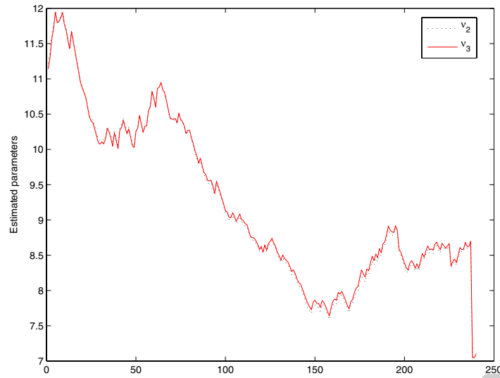
Fig. 1. Recursive estimates of \hat{\nu}_2 and \hat{\nu}_3 for the out-of-sample period.
