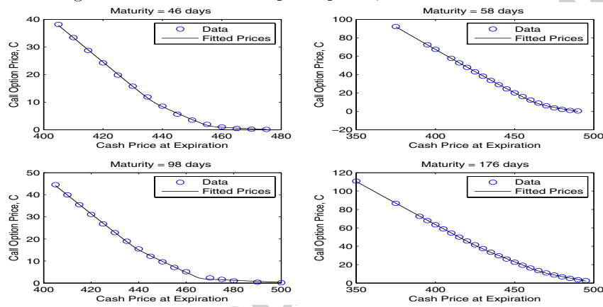
Fig. 4. Actual and fitted option prices, scaled and shifted t .
