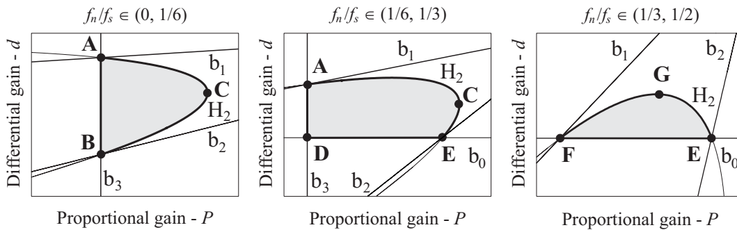
Fig. 3: Possible shapes of the P - d stability charts
