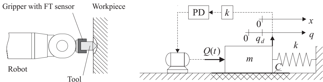
Fig. 1: Mechanical model of unidirectional PD force control
