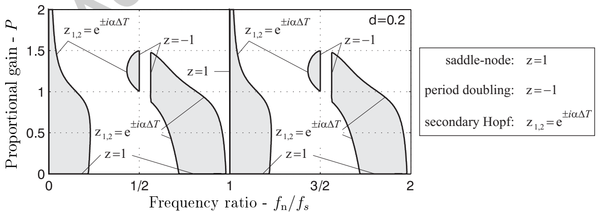
Fig. 5: The three different kinds of possible bifurcations
