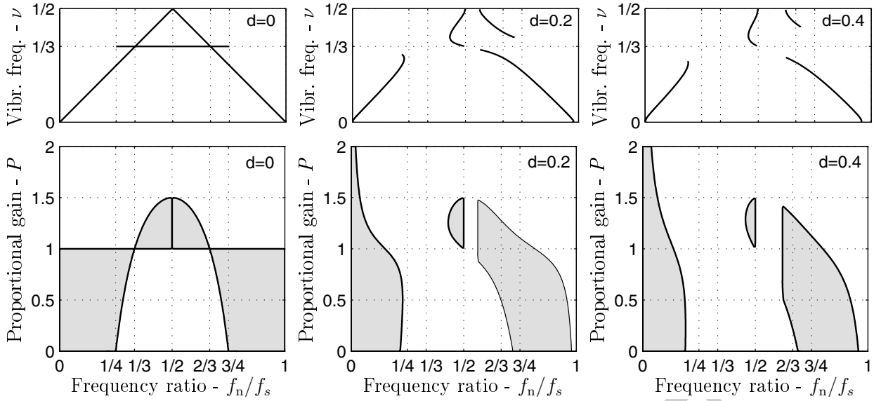
Fig. 4: The f_n/f_s - P stability charts
