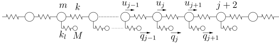
Fig. 1. Spring mass system with attached local oscillators.
