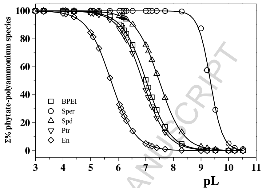
Figure 3 Sum of percentages of phytate-polyammonium cations species vs. pL at I = 0 \text{ mol L}^{-1} , t = 25 \text{ }^\circ\text{C} and \text{pH} = 7.4 . Concentration: C_{\text{polyammonium cation}} = (\text{trace}) .
