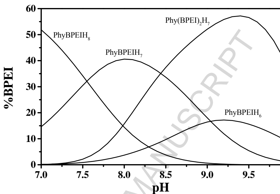
Figure 2. Speciation diagram for the species of phytate-BPEI system at I = 0 \text{ mol L}^{-1} and t = 25 \text{ }^\circ\text{C} . Experimental condition: C_{\text{BPEI}} = 1 \text{ mmol L}^{-1} and C_{\text{phytate}} = 1.5 \text{ mmol L}^{-1} .
