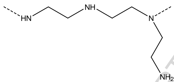
Figure 1. Representation of BPEI monomeric unit.
