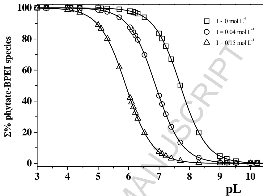
Figure 4 Sum of percentages of phytate-BPEI species vs. pL at different ionic strengths at pH = 7.4 and t = 25 °C. Concentration: C_{\text{BPEI}} = (\text{trace}) .
