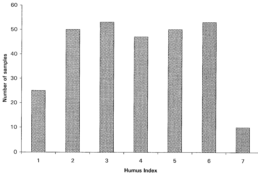
Fig. 1. Distribution of the seven humus index classes among the 288 humus profiles studied.
