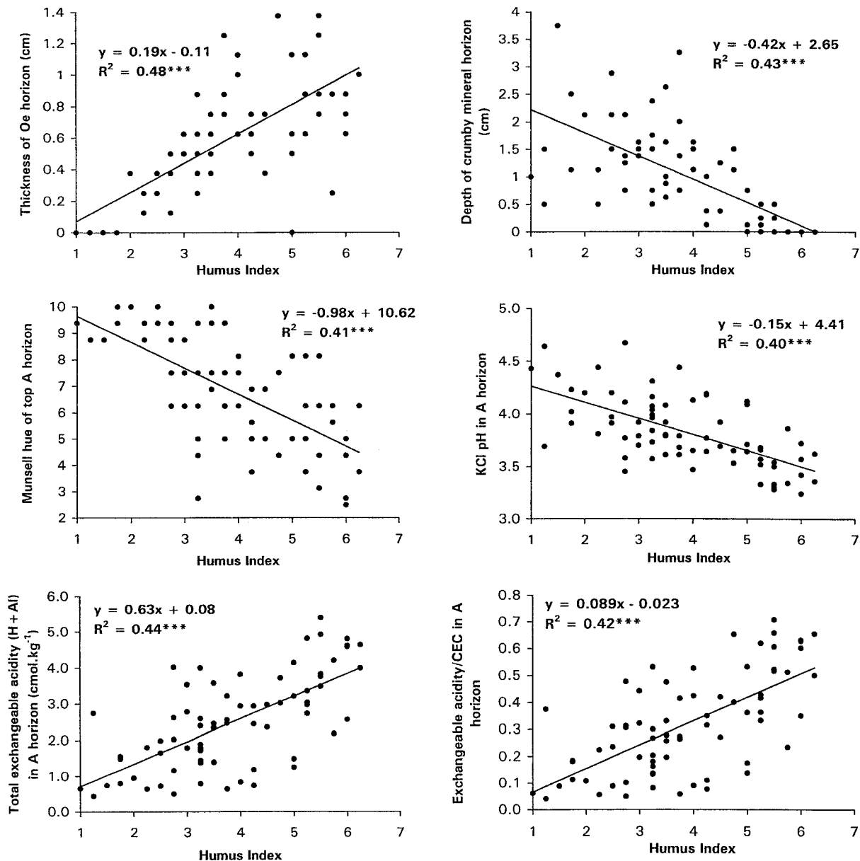
Fig. 2. Correlation of the humus index with some variables measured in the topsoil profiles (means of four replicates).
