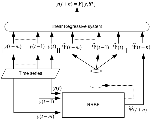
Figure 5. “ t+n ” step-ahead-prediction obtained by the NARX model (the whole model)
