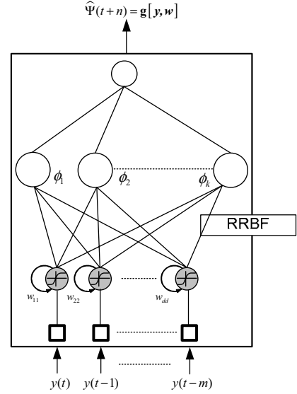
Figure 2. “ t+n ” step-ahead-prediction obtained by the Neural Network
