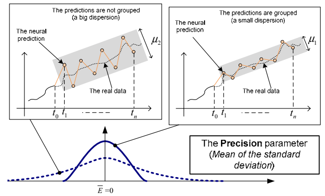
Figure 7. an example of two different Precision values.
