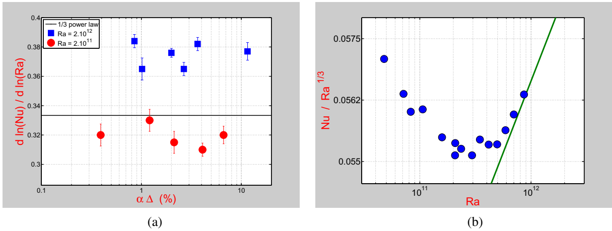
Figure A.2. (a) Local exponent of the Nu(Ra) dependence versus the non-Boussinesq parameter \alpha \Delta . The Rayleigh numbers Ra = 2 \times 10^{11} and 2 \times 10^{12} were chosen on each side of the transition to the Ultimate Regime. (b) Evidence of the transition at a mean density of 18.69 \text{ kg m}^{-3} and a mean temperature of 11.4 \text{ K} , that is, at about a quarter of the critical density and at twice the critical temperature.
