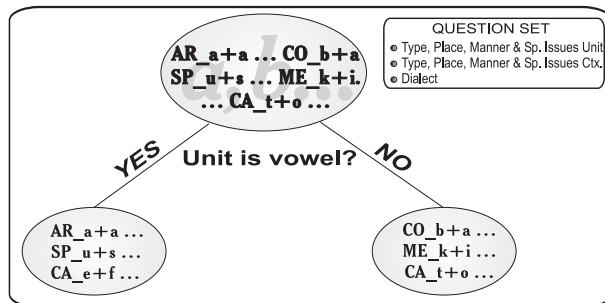
(b) Dialect-context-dependent models, one-root tree structure (DCD-OR)
