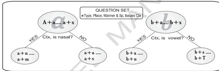
(a) Global phone set, multiroot tree structure (GPS-MR)
