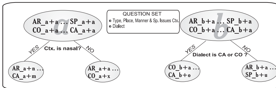
(a) Dialect-context-dependent models, multiroot tree structure (DCD-MR)
