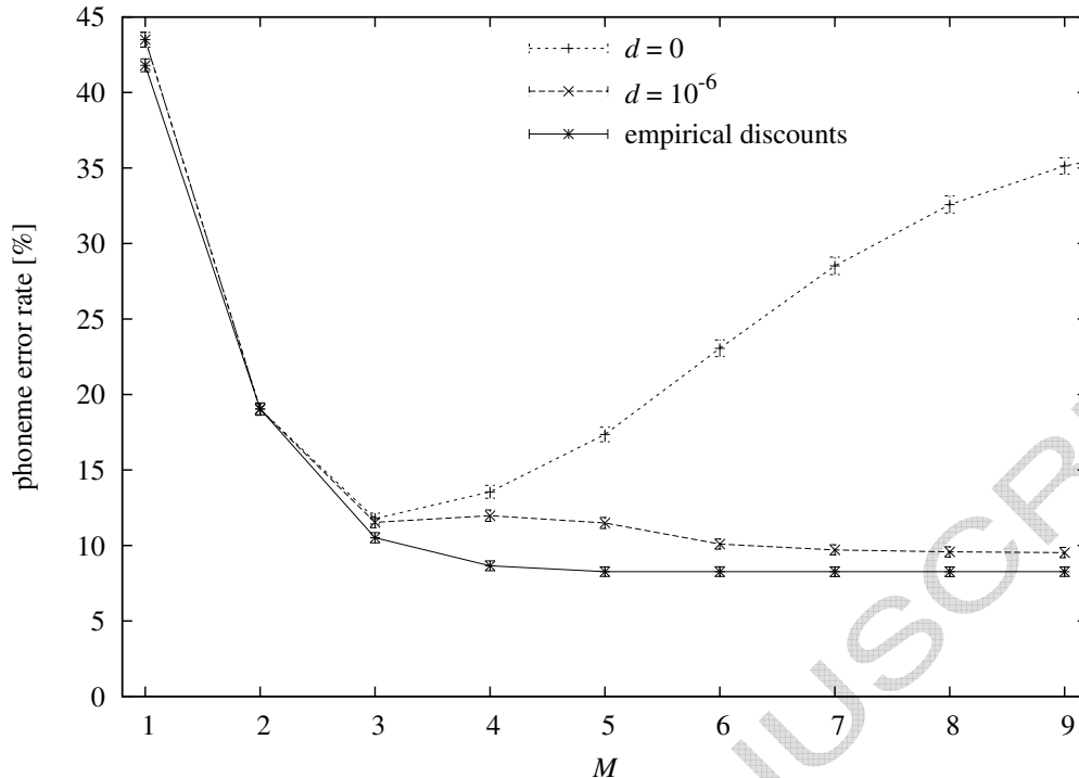
Fig. 5. Grapheme-to-phoneme conversion accuracy on the NETtalk 15k for smoothed and unsmoothed models as a function of context length ( L = 1 ). Error bars show 90% confidence intervals.
