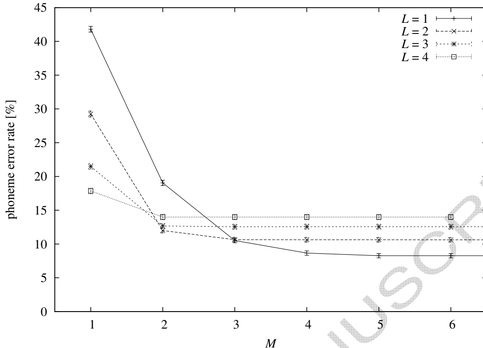
Fig. 3. Grapheme-to-phoneme conversion performance on the NETtalk 15k data set for L -to- L models of different complexities. Error bars show 90% confidence intervals.
