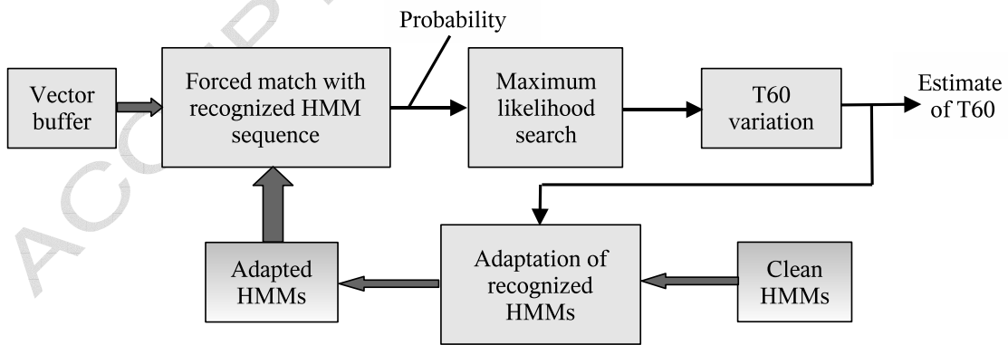
Figure 5: Estimation of T60 by an iterative search of the maximum likelihood
