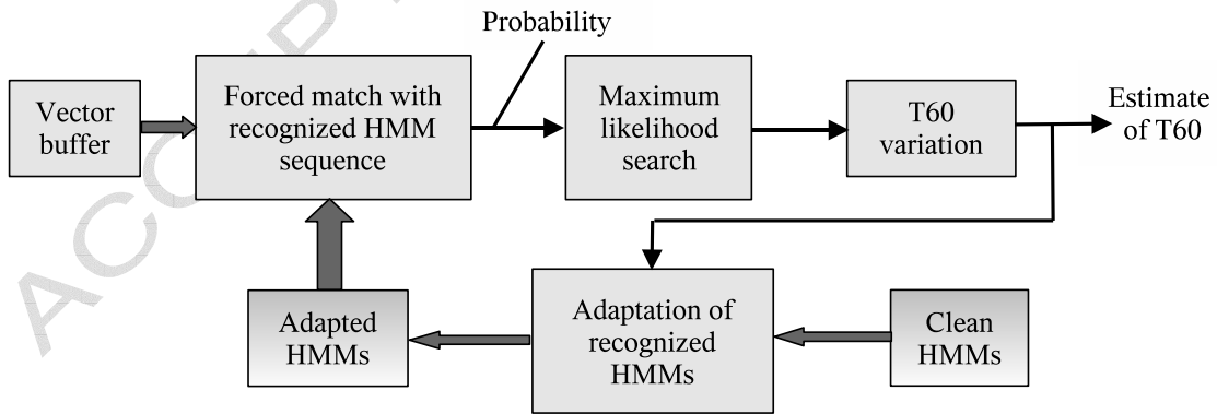
Figure 5: Estimation of T60 by an iterative search of the maximum likelihood
