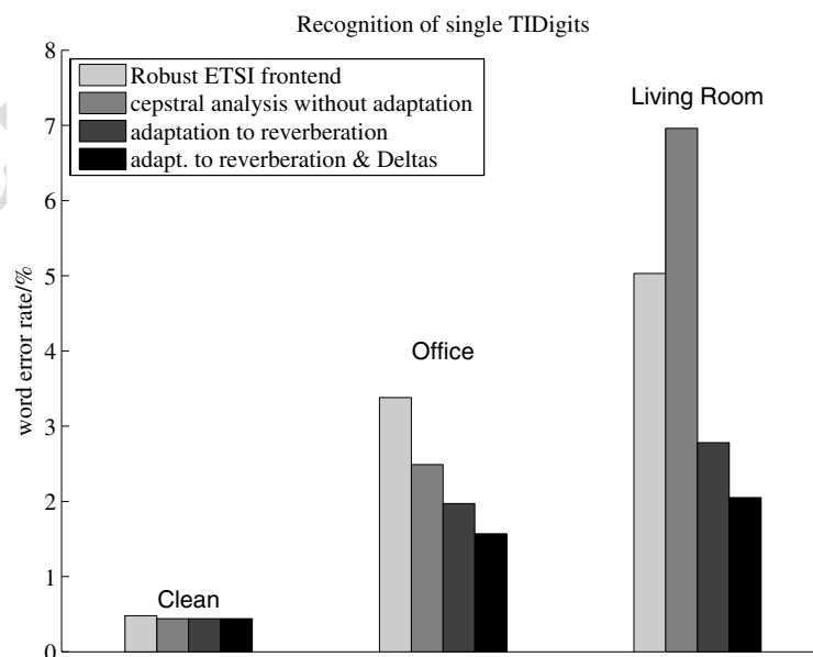
Figure 8: Word error rates for these TIDigits utterances that contain only single digits
