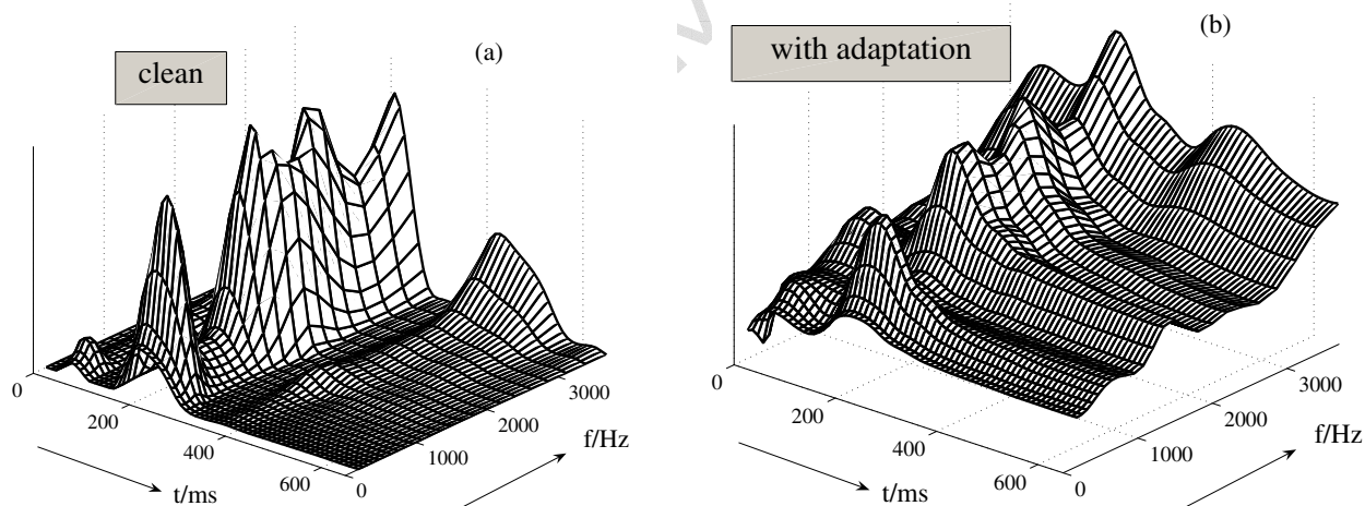
Figure 12: Spectrograms of the clean and the adapted HMMs for the word “six”
