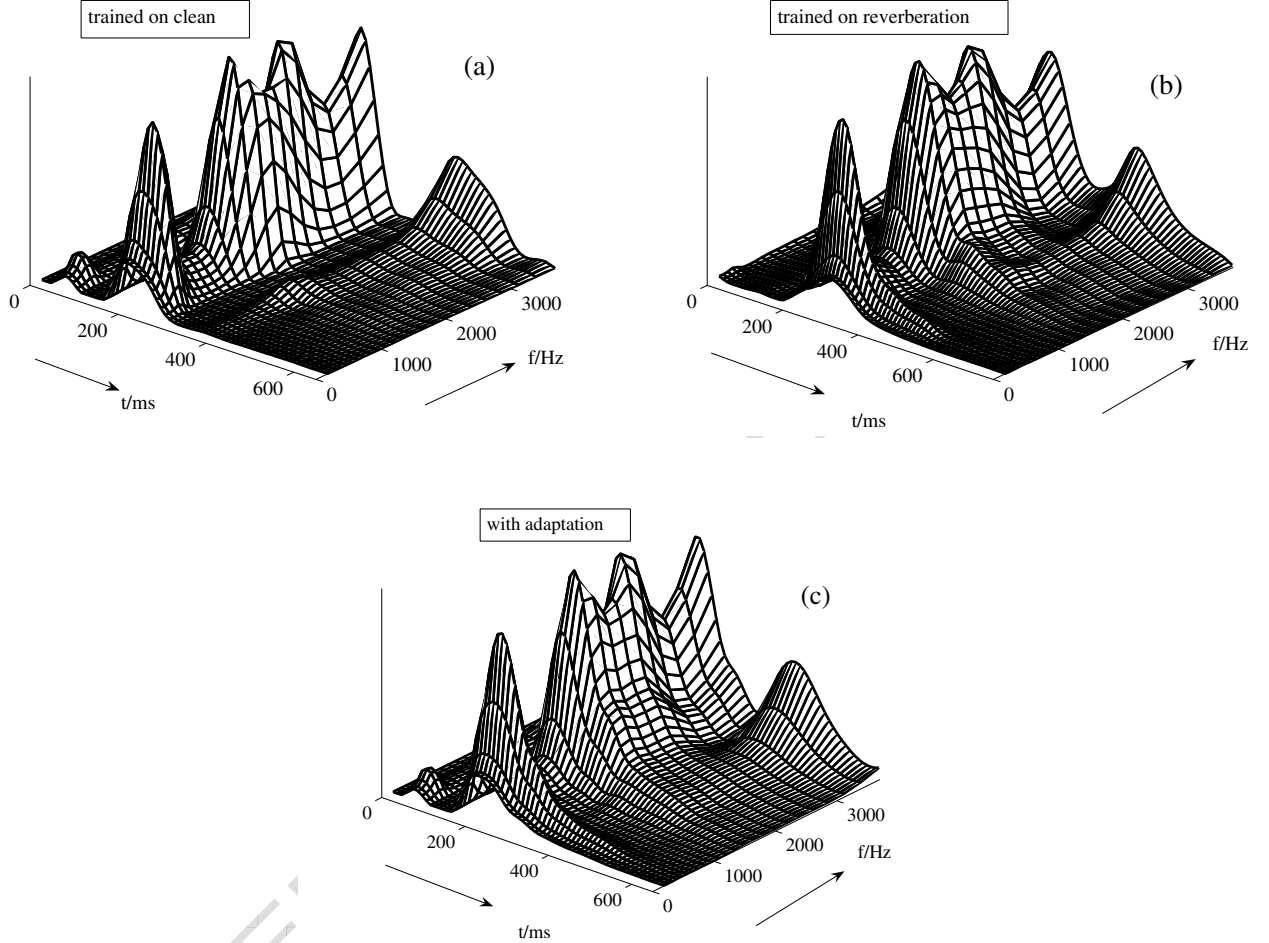
Figure 4: Different spectrograms of HMMs for the word “six”
