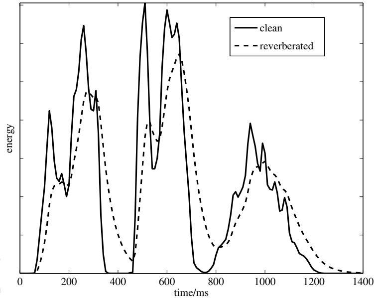
Figure 1: Energy contours of a speech signal in clean and reverberant condition
