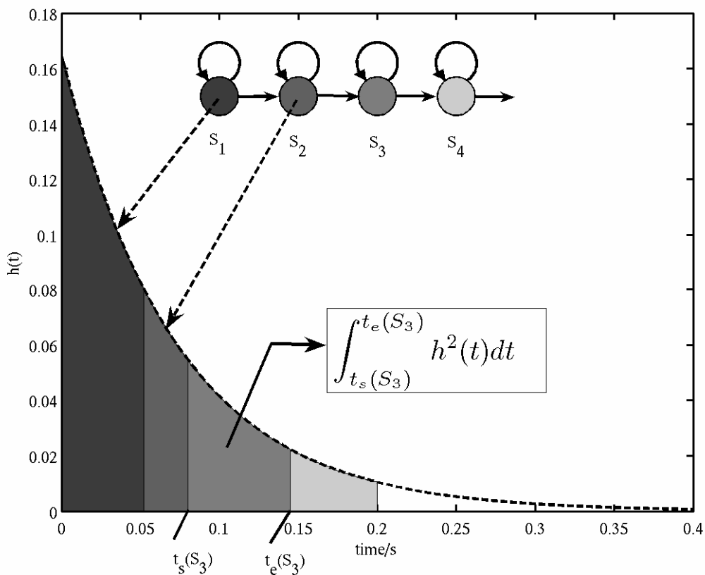
Figure 3: The distribution of energy at state S_1 due to reverberation
