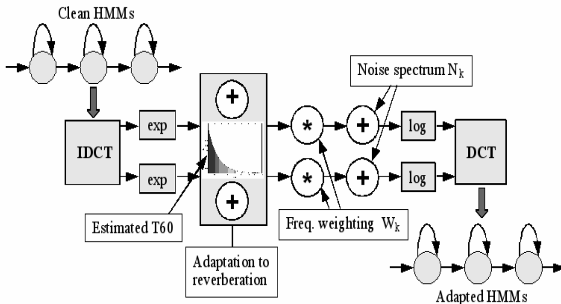
Figure 11: Scheme for adapting HMMs to all distortion effects
