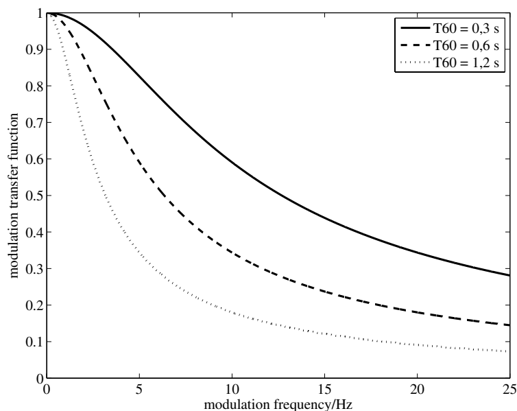
Figure 2: Modulation transfer functions for different values of T_{60}
