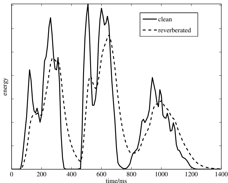
Figure 1: Energy contours of a speech signal in clean and reverberant condition
