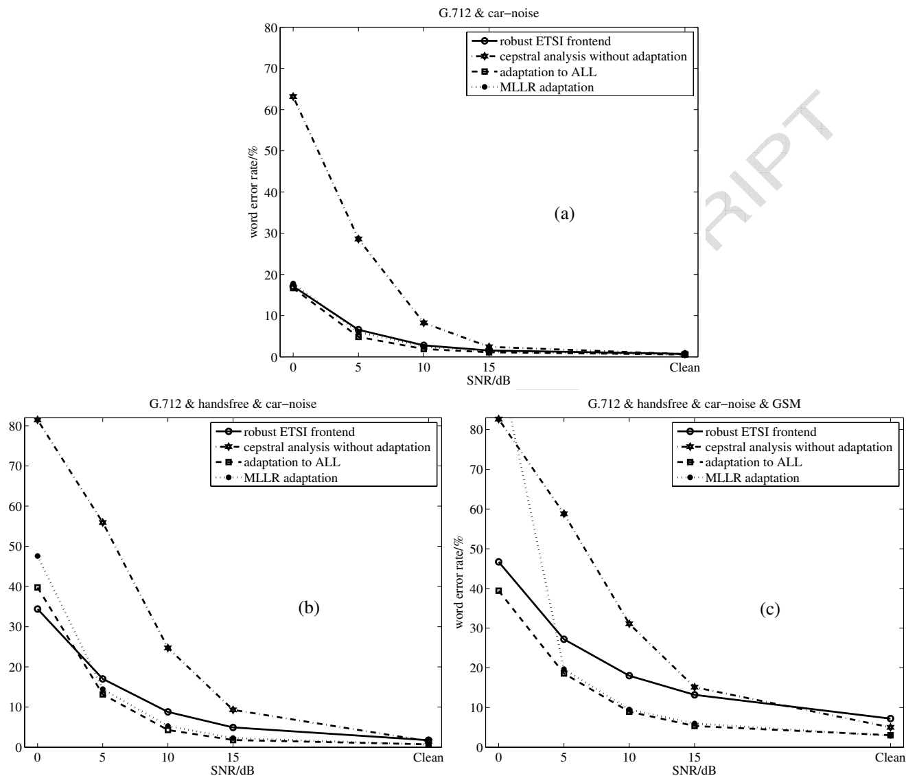
Figure 13: Word error rates for different recording conditions inside a car
