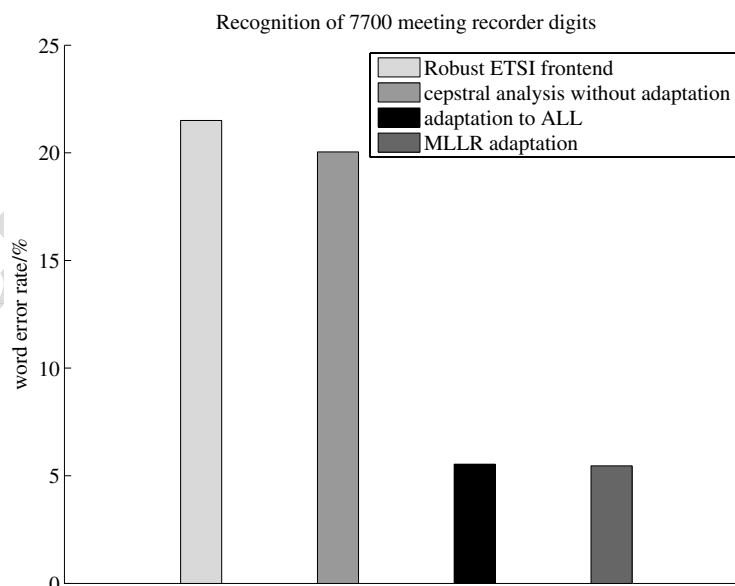
Figure 16: Word error rates for the meeting recorder digits with HMMs trained on TIDigits
