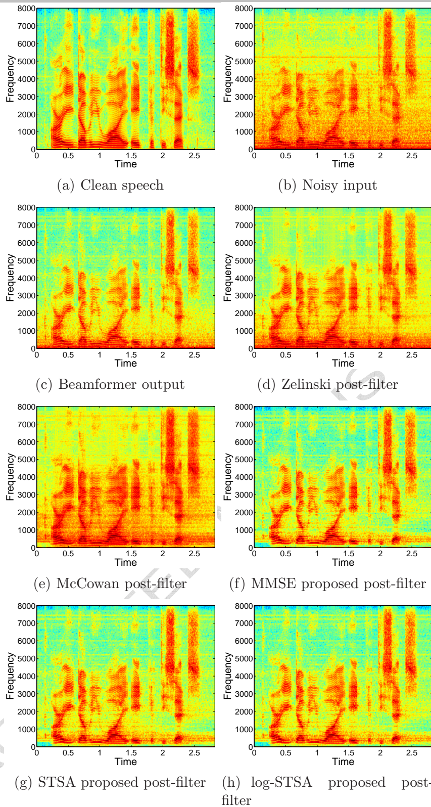
Fig. 3. Speech Spectrograms for an utterance “r-e-w-y-8-56”. (a) Original clean speech. (b) Noisy signal at central sensor (IS=1.44). (c) Beamformer output (SSNRE=0.02 dB, IS=0.90). (d) Zelinski post-filter (SSNRE=0.17 dB, IS=2.89). (e) McCowan post-filter (SSNRE=3.95 dB, IS=2.08). (f) MMSE (SSNRE=4.54 dB, IS=0.81). (g) STSA (SSNRE=4.46 dB, IS=0.82). (h) log-STSA (SSNRE=4.52 dB, IS=0.81).
