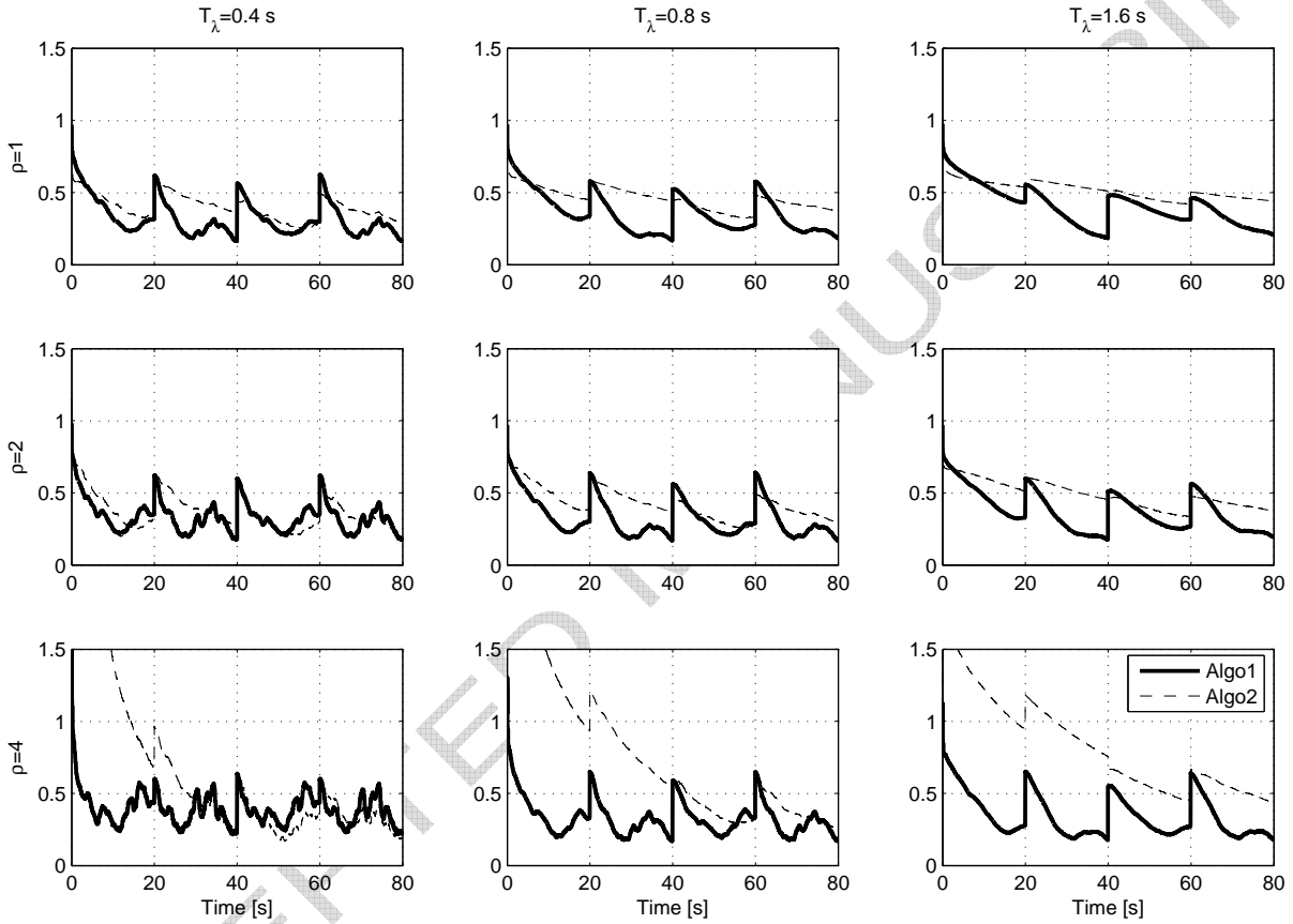
Fig. 12. Filter convergence \Delta \mathbf{w}[m] of SDR-GSC for a switching speech scenario (unconstrained update, 1/\mu = 0.5 , mismatch, perfect VAD).
