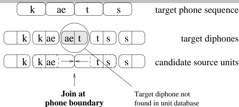
Fig. 2. An illustration of using phone boundary joins to deal with isolated instances in the target diphone sequence which are missing in the voice database. In this example, the [\text{æ}]-[\text{t}] diphone required to synthesise the word “cats” is missing. In order to compensate for this, the margins of the directly neighbouring diphone source units can be extended as shown. This results in the inclusion of whole [\text{æ}] and [\text{t}] phones from the voice database, with the join at the phone boundary between them instead of the usual diphone boundary.
