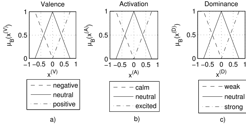
Fig. 3. Membership functions of the emotion components.
