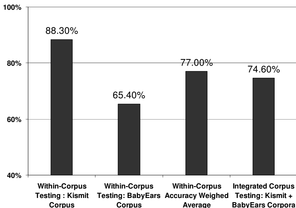
Fig. 3. Comparison of the classification accuracies obtained in different settings.
