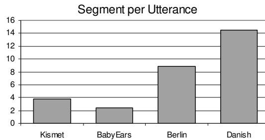
Fig. 2: Average Number of Voiced Segments per Utterance in the Four Databases
