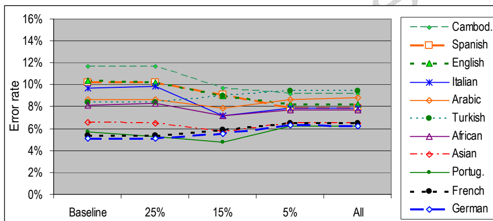
Figure 4 – Error rates for each language group using phonological rules and various selections of foreign-adapted units.
