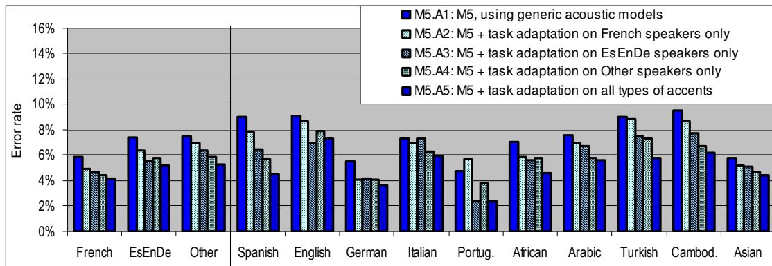
Figure 7 – Error rates for each language group for the best modeling variant, after various accents adaptation.
