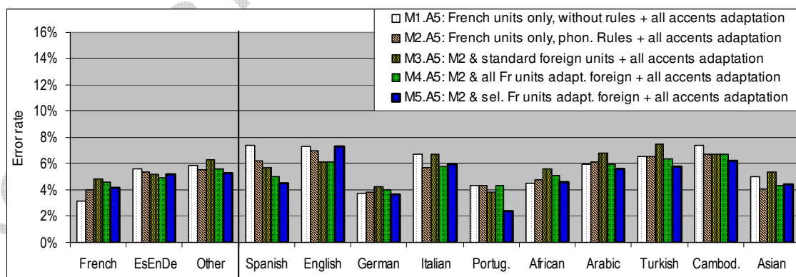
Figure 6 – Error rates for each language group for baseline and modeling variants, after task and accent adaptation.
