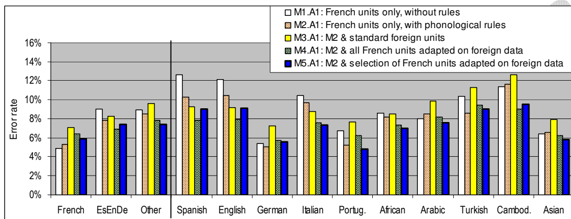
Figure 3 – Error rates for each language group for baseline and modeling variants, before task and accent adaptation.
