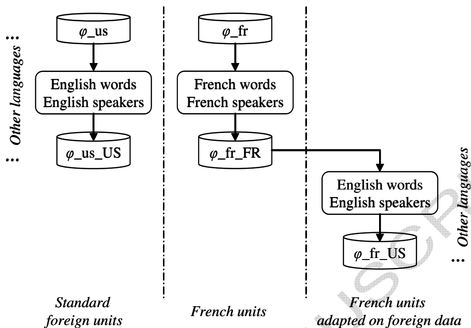
Figure 2 – Training scheme for standard foreign units (left) and French units adapted on foreign data (right).
