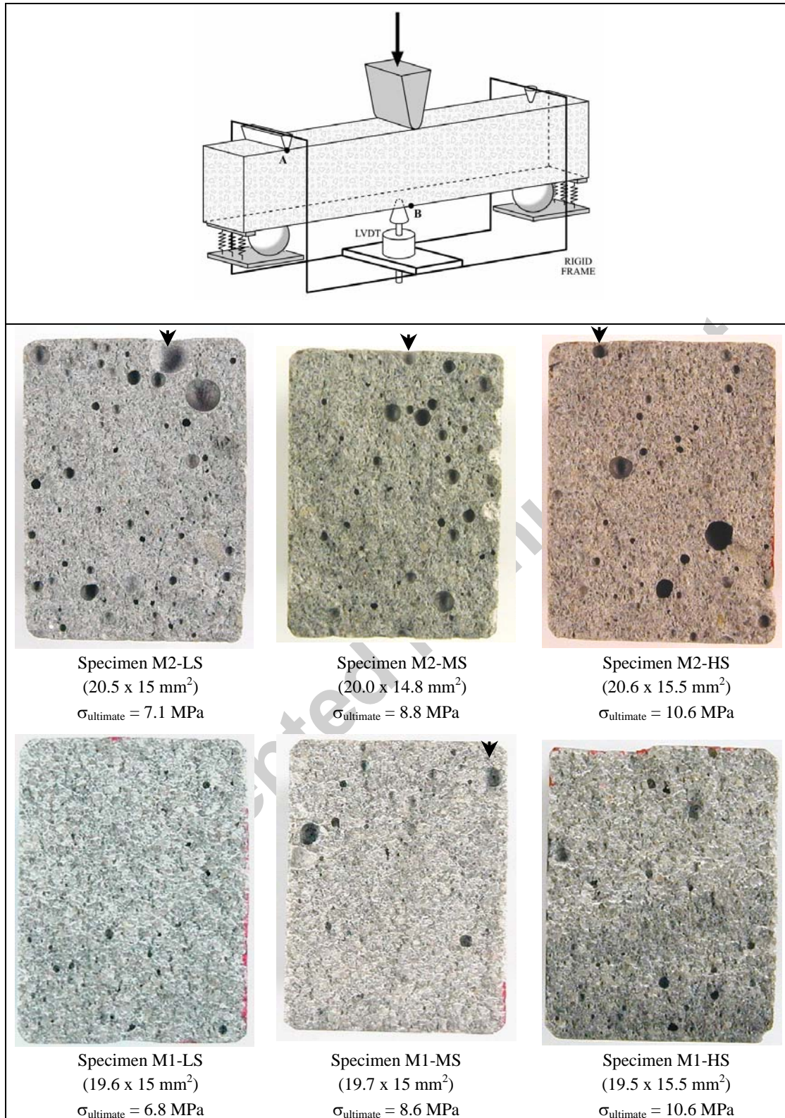
Figure 3. Top: sketch of three-point bending device. Bottom: fracture surface of three M2 specimens and three M1 specimens after bending tests
