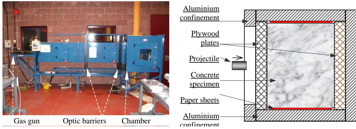
Figure 6. Gas gun and sarcophagus set-up used for the impact test
