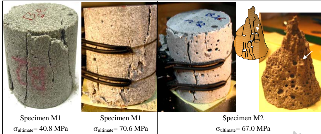
Figure 4. Specimens M1 and M2 after failure, simple compression tests
