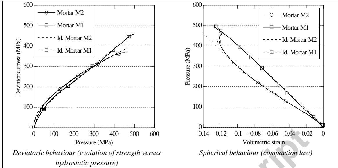
Figure 11. Fitting the KST-model parameters with the deviatoric and spherical behaviours of mortars M1 and M2. ("Id." curves: curves identified for the KST model)
