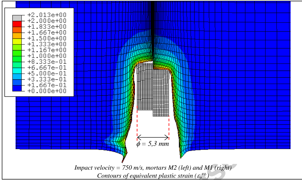
Figure 12. Numerical simulations of the impact test using the KST model (parameters identified from Figure 11)
