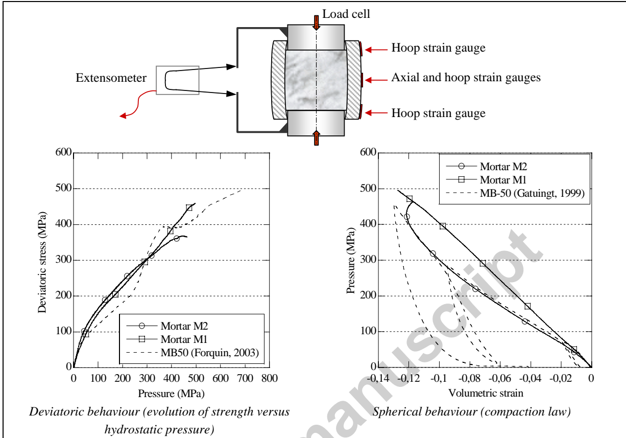
Figure 5. Top: sketch of the device used for quasi-oedometric compression tests. Bottom: experimental results obtained with mortars M1, M2 and compared with that of concrete MB50 [35,36]
