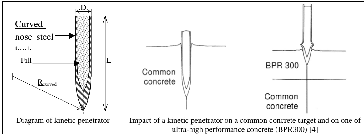
Figure 1. Impact of a kinetic penetrator on a thick concrete target
