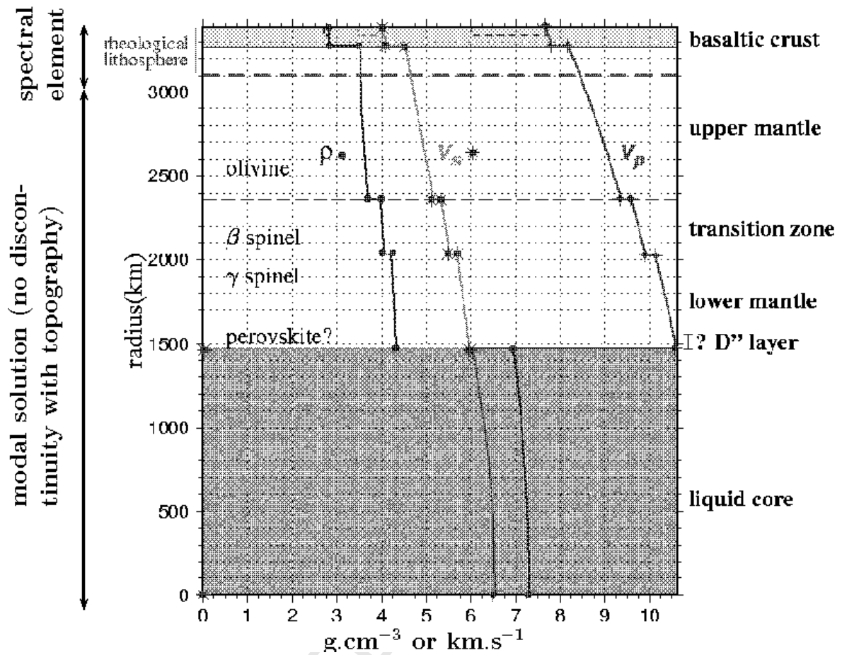
FIGURE 2 C. Larmat et al. , 2006. Effects of the martian crust on seismograms.
