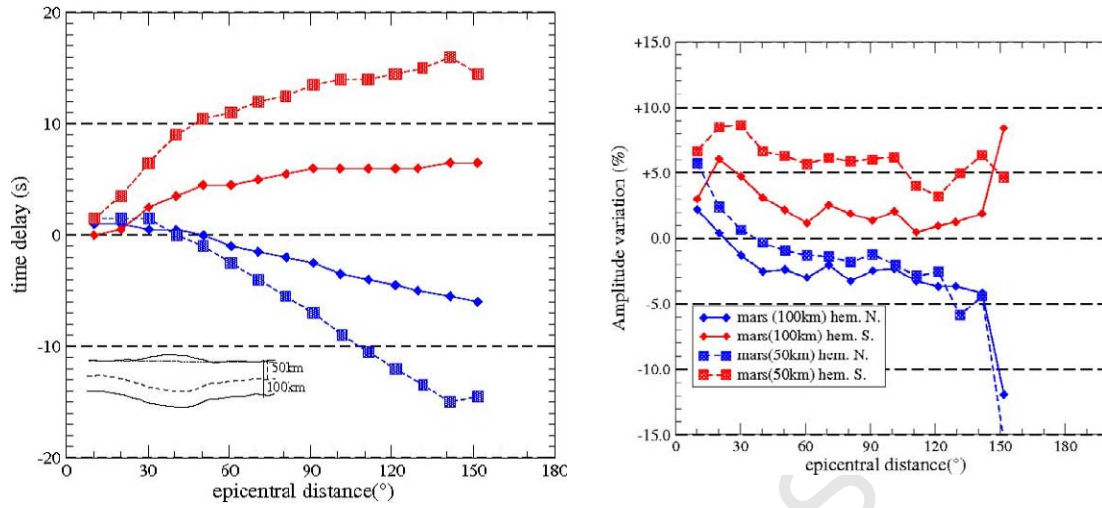
FIGURE 8 C. Larmat et al , 2006. Effects of the martian crust on seismograms.
