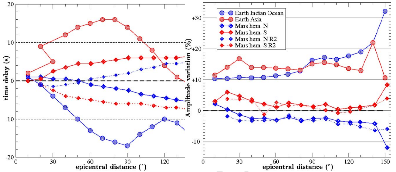
FIGURE 7 C. Larmat et al. , 2006. Effects of the martian crust on seismograms.
