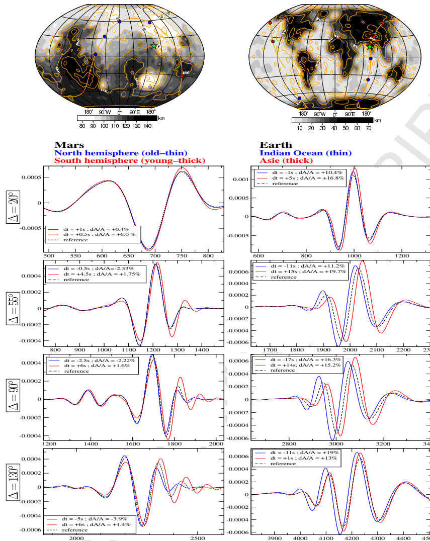
FIGURE 6 C. Larmat et al , 2006. Effects of the martian crust on seismograms.
