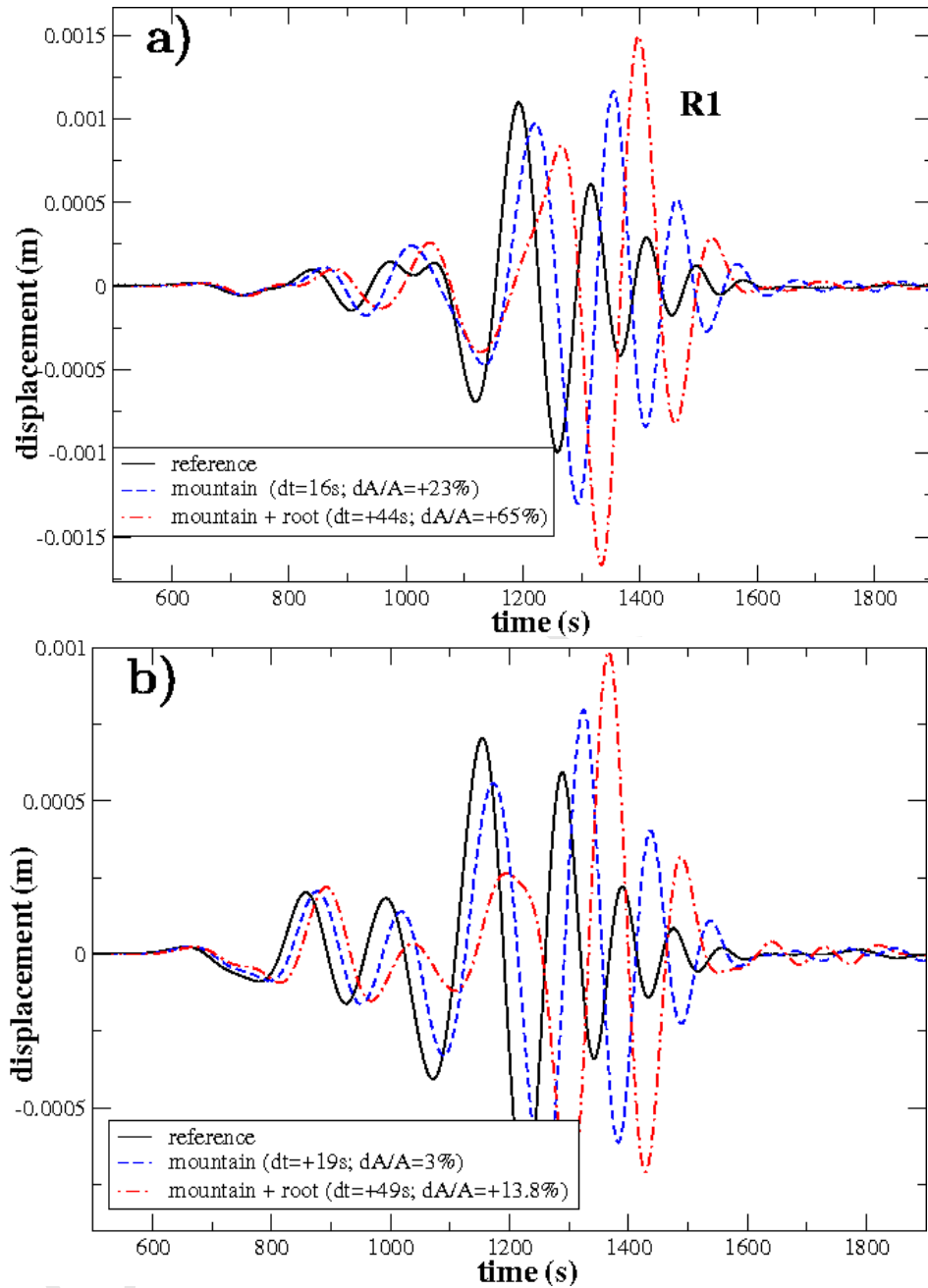
FIGURE 5 C. Larmat et al. , 2006. Effects of the martian crust on seismograms.
