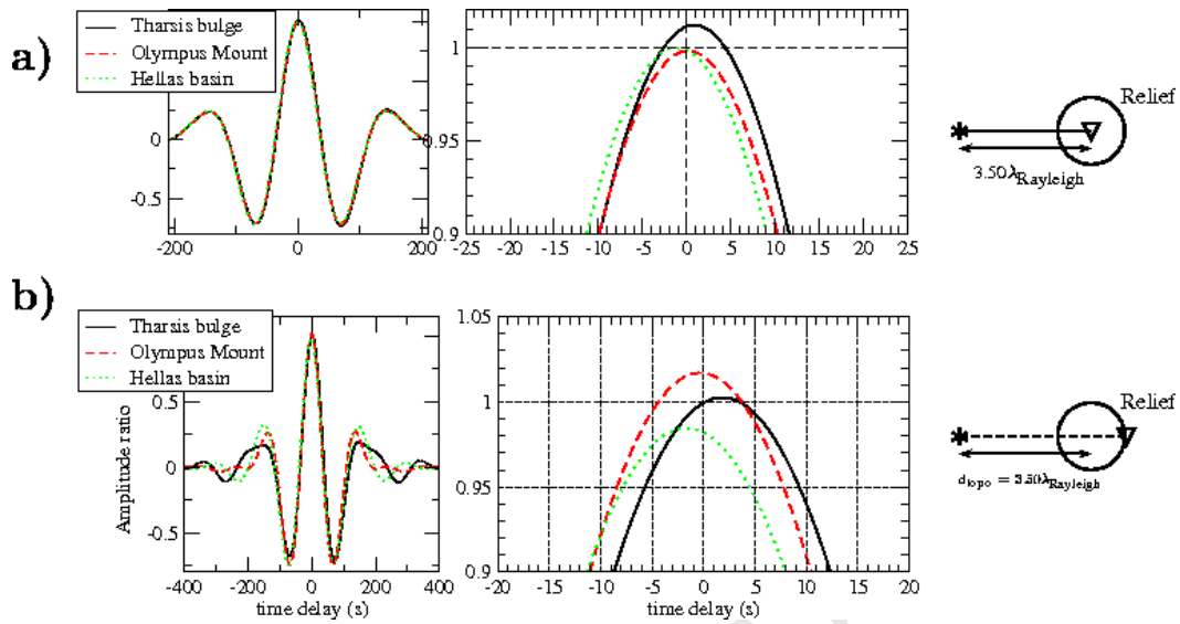
FIGURE 3 C. Larmat et al. , 2006. Effects of the martian crust on seismograms.
