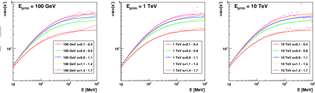
Fig. 4. Mean value of scaled angle \langle w \rangle (s) as function of particle energy and shower age, for different primary particle energies (100 GeV to 10 TeV from left to right). The solid lines correspond to the parametrization of eq. 8. The average scaled particle angle is found to be mostly independent of primary particle energy.
