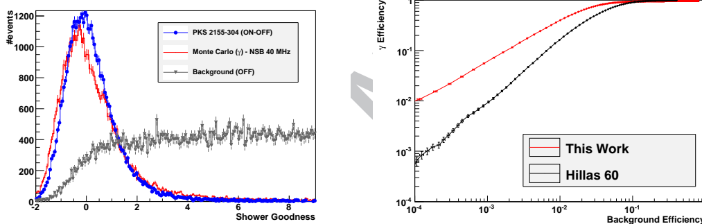
Fig. 19. Left: Distribution of Shower Goodness for real data taken on the blazar PKS 2155-304 (blue point for excess events, grey triangles for background events), compared with a simulation (red histogram) with a similar night sky background level. Right: \gamma -ray efficiency as function of background rejection for a selection based on Shower Goodness, compared with selection achieved in a standard Hillas parameters reconstruction at the same minimum image amplitude (60 p.e.) and with the Mean Scaled Width and Mean Scaled Length variables.
